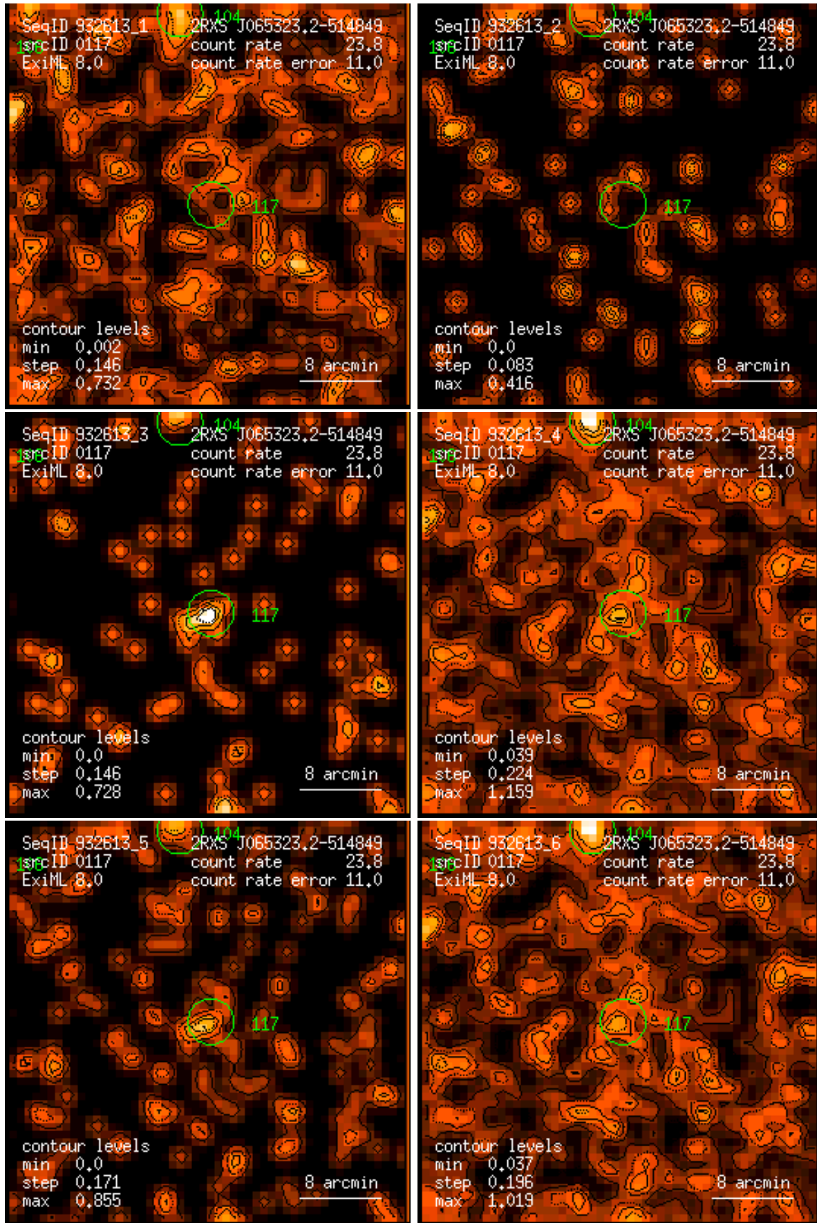
Figure 117: RASS 932613: detection 0117: band rate images, Gaussian filter: (1) PSPC channels 11 – 41, (2) 52 – 90, (3) 91 – 201, (4) 11 – 235, (5) 52 – 201, (6) 11 – 201. Broad band rates in counts/ks. Band rate contour levels in counts/ks/arcmin 2 .
