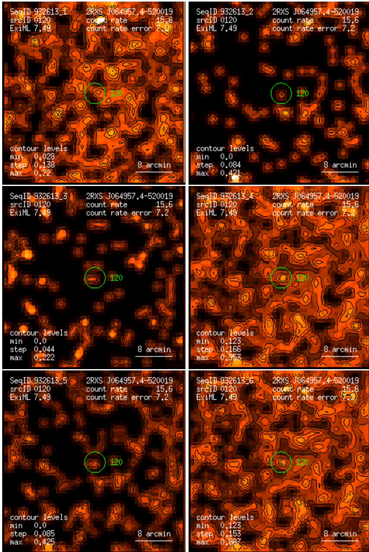
Figure 120: RASS 932613: detection 0120: band rate images, Gaussian filter: (1) PSPC channels 11 – 41, (2) 52 – 90, (3) 91 – 201, (4) 11 – 235, (5) 52 – 201, (6) 11 – 201. Broad band rates in counts/ks. Band rate contour levels in counts/ks/arcmin 2 .
