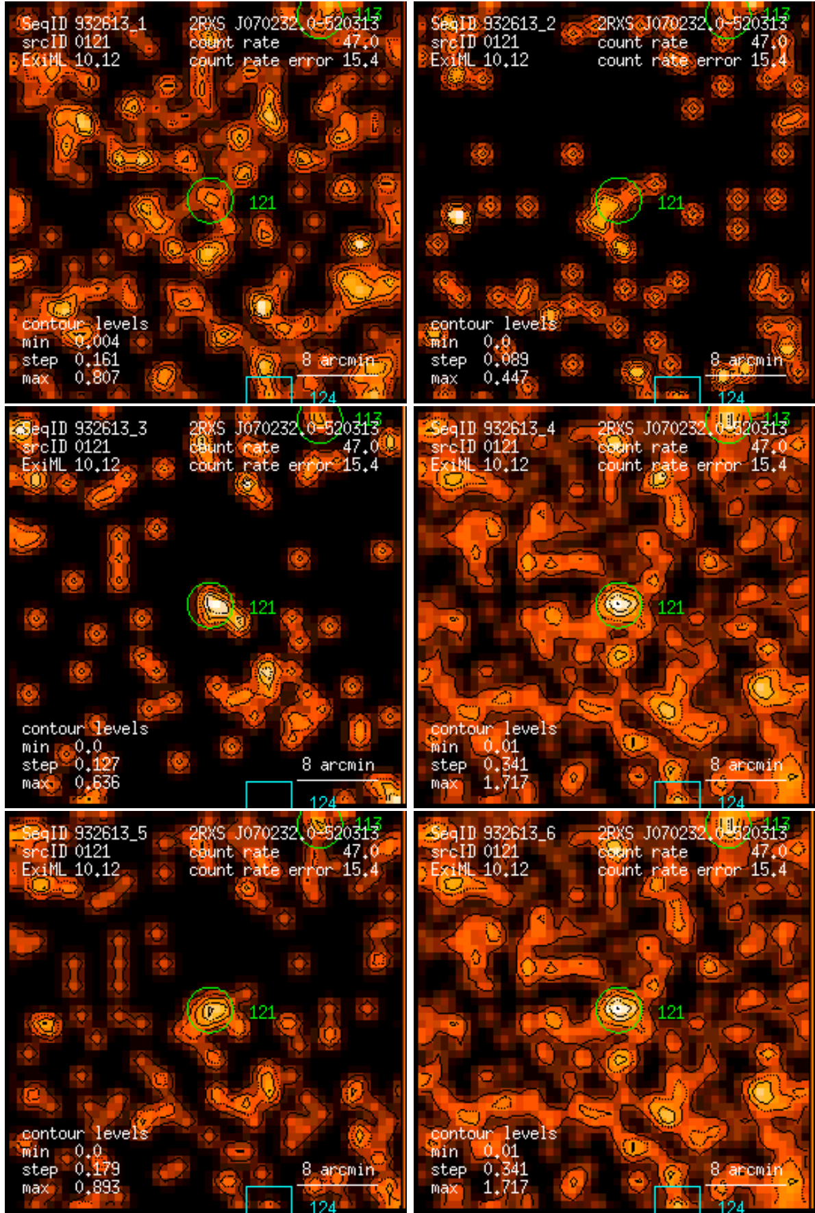
Figure 121: RASS 932613: detection 0121: band rate images, Gaussian filter: (1) PSPC channels 11 – 41, (2) 52 – 90, (3) 91 – 201, (4) 11 – 235, (5) 52 – 201, (6) 11 – 201. Broad band rates in counts/ks. Band rate contour levels in counts/ks/arcmin 2 .
