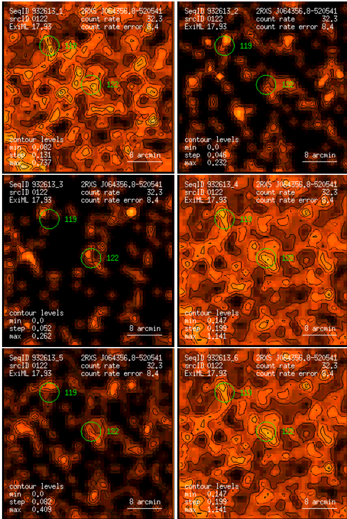
Figure 122: RASS 932613: detection 0122: band rate images, Gaussian filter: (1) PSPC channels 11 – 41, (2) 52 – 90, (3) 91 – 201, (4) 11 – 235, (5) 52 – 201, (6) 11 – 201. Broad band rates in counts/ks. Band rate contour levels in counts/ks/arcmin 2 .
