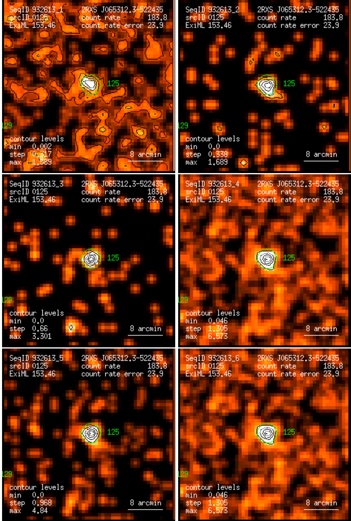
Figure 125: RASS 932613: detection 0125: band rate images, Gaussian filter: (1) PSPC channels 11 – 41, (2) 52 – 90, (3) 91 – 201, (4) 11 – 235, (5) 52 – 201, (6) 11 – 201. Broad band rates in counts/ks. Band rate contour levels in counts/ks/arcmin 2 .
