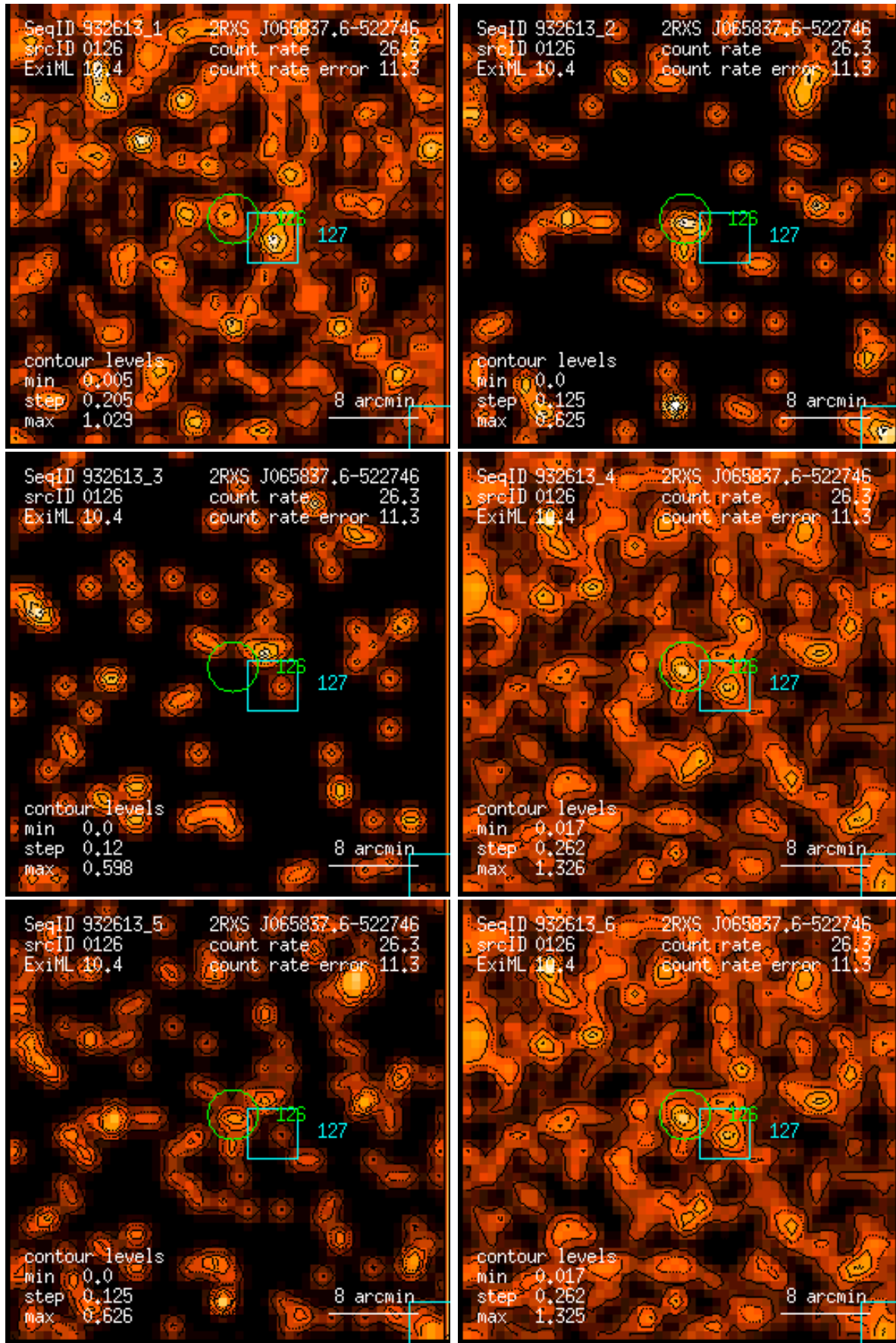
Figure 126: RASS 932613: detection 0126: band rate images, Gaussian filter: (1) PSPC channels 11 – 41, (2) 52 – 90, (3) 91 – 201, (4) 11 – 235, (5) 52 – 201, (6) 11 – 201. Broad band rates in counts/ks. Band rate contour levels in counts/ks/arcmin 2 .
