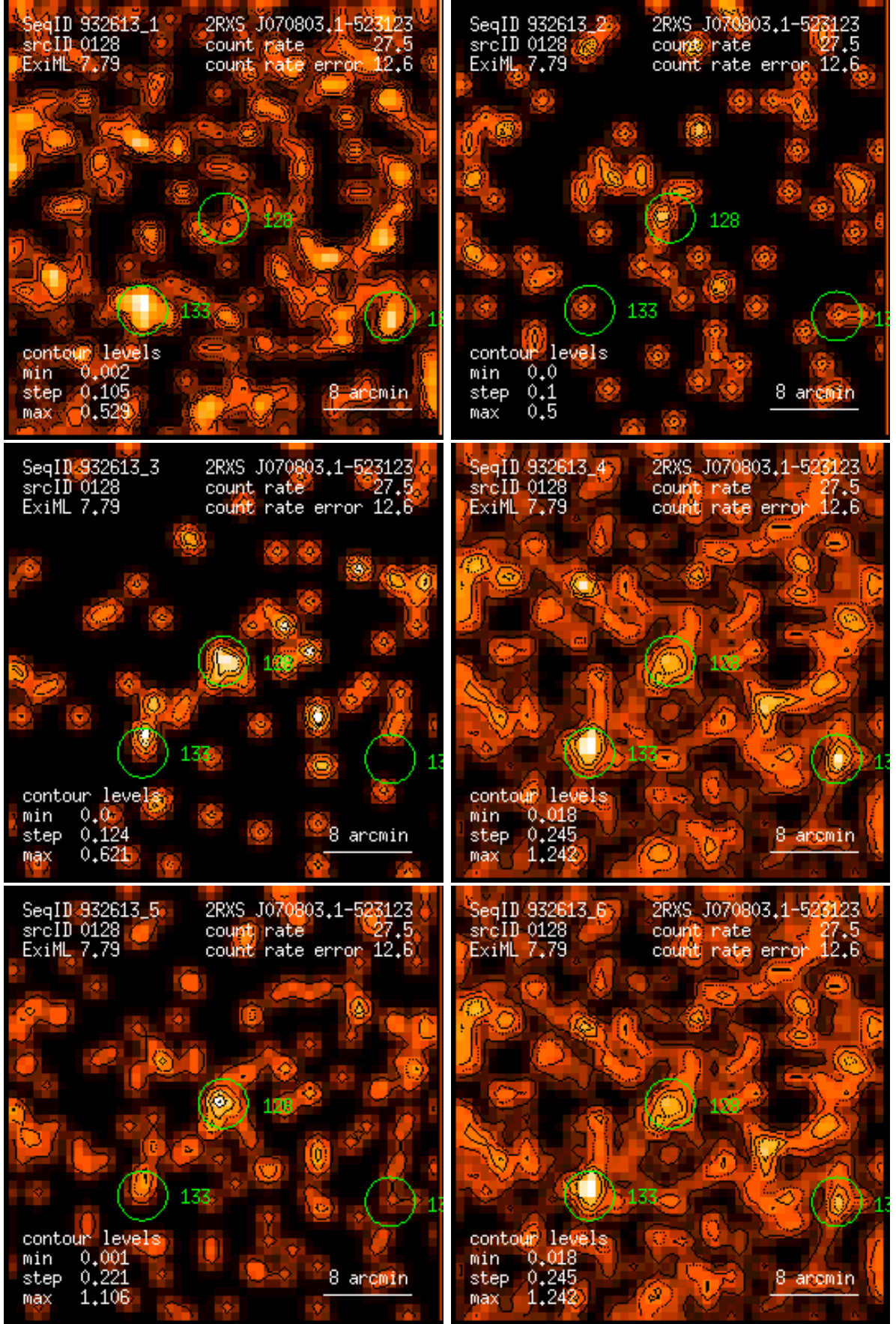
Figure 128: RASS 932613: detection 0128: band rate images, Gaussian filter: (1) PSPC channels 11 – 41, (2) 52 – 90, (3) 91 – 201, (4) 11 – 235, (5) 52 – 201, (6) 11 – 201. Broad band rates in counts/ks. Band rate contour levels in counts/ks/arcmin 2 .
