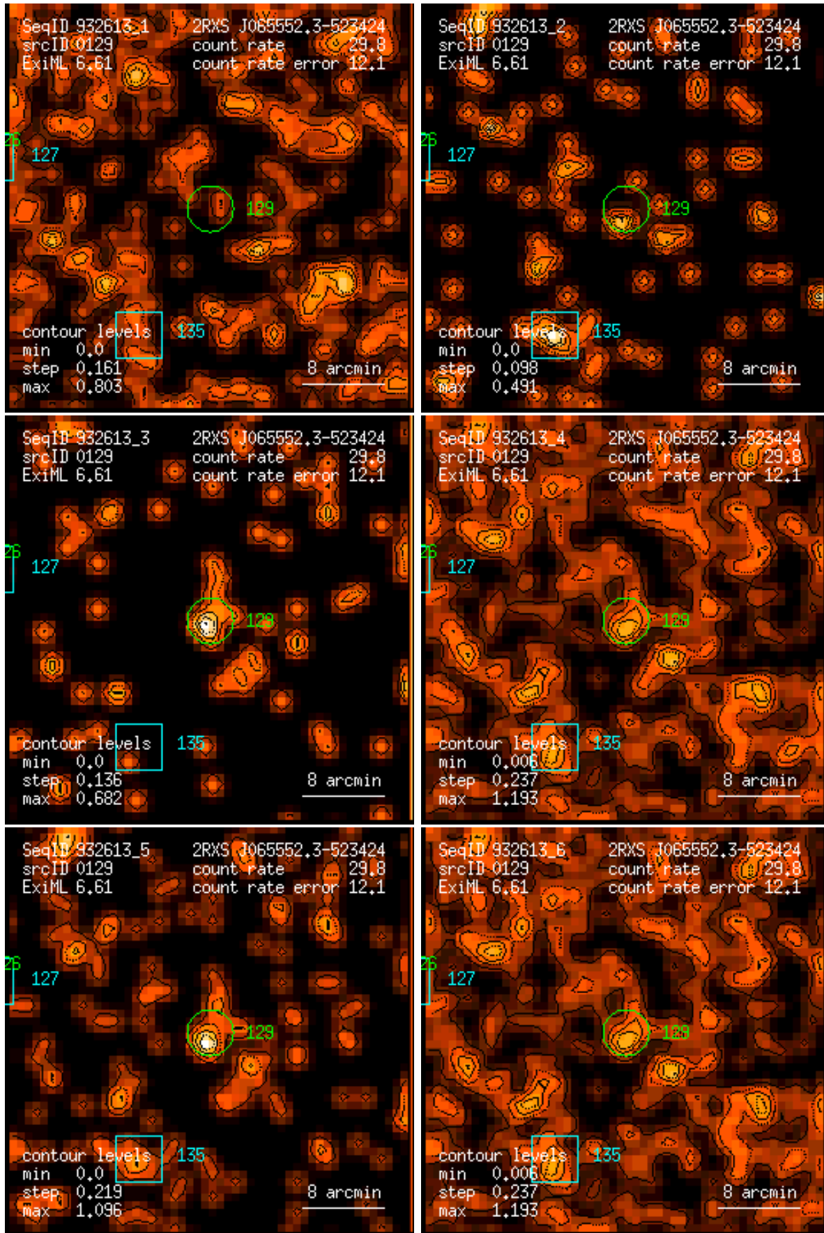
Figure 129: RASS 932613: detection 0129: band rate images, Gaussian filter: (1) PSPC channels 11 – 41, (2) 52 – 90, (3) 91 – 201, (4) 11 – 235, (5) 52 – 201, (6) 11 – 201. Broad band rates in counts/ks. Band rate contour levels in counts/ks/arcmin 2 .
