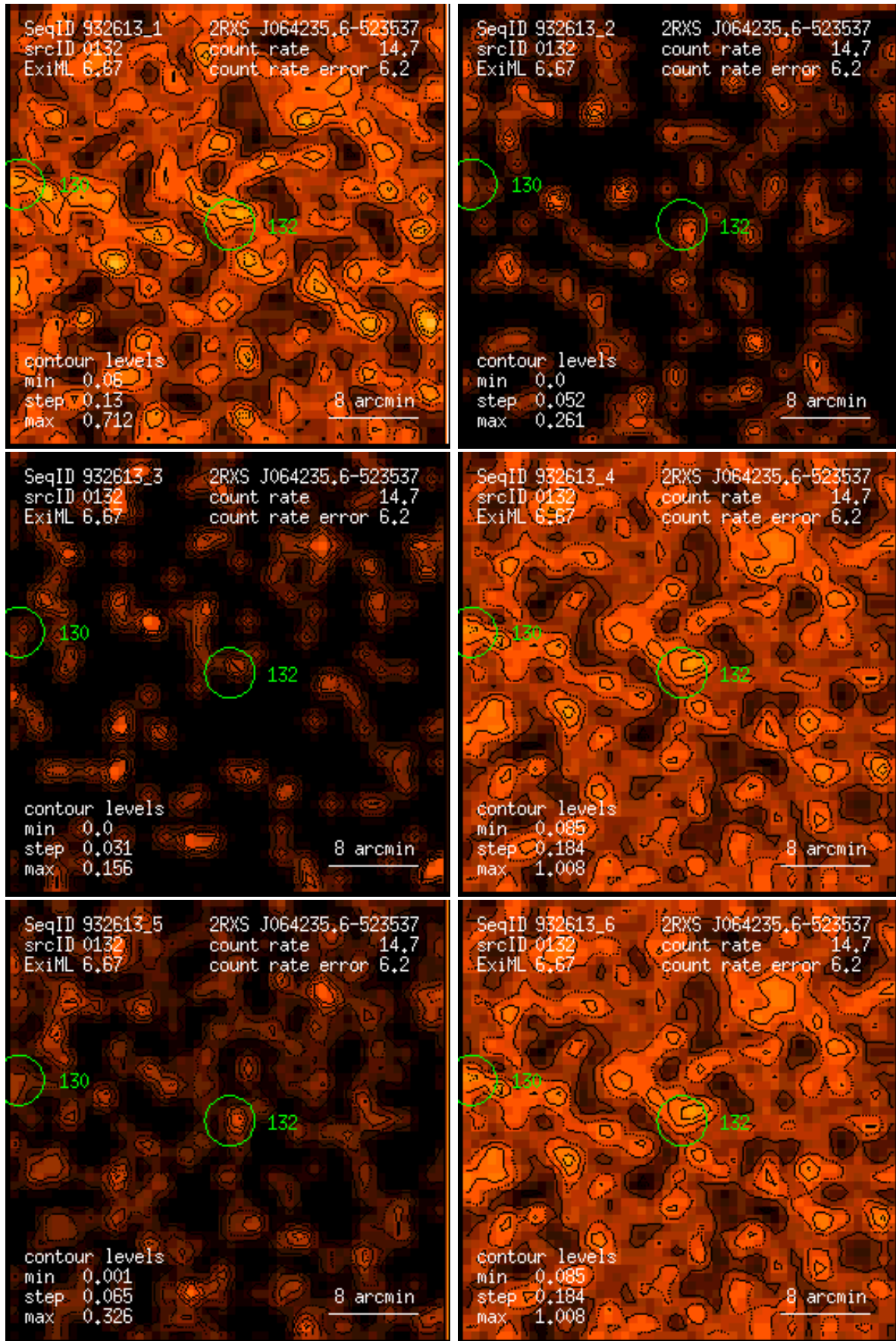
Figure 132: RASS 932613: detection 0132: band rate images, Gaussian filter: (1) PSPC channels 11 – 41, (2) 52 – 90, (3) 91 – 201, (4) 11 – 235, (5) 52 – 201, (6) 11 – 201. Broad band rates in counts/ks. Band rate contour levels in counts/ks/arcmin 2 .
