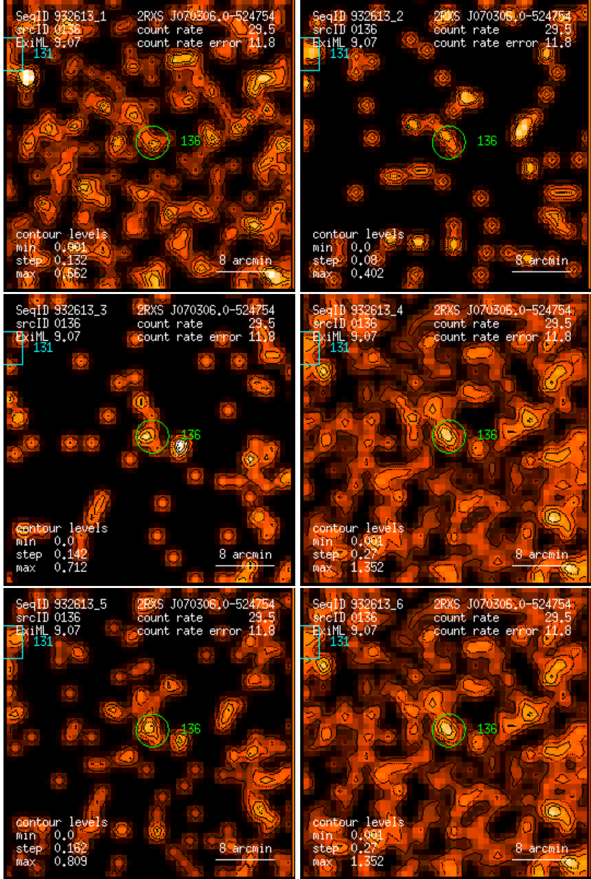
Figure 136: RASS 932613: detection 0136: band rate images, Gaussian filter: (1) PSPC channels 11 – 41, (2) 52 – 90, (3) 91 – 201, (4) 11 – 235, (5) 52 – 201, (6) 11 – 201. Broad band rates in counts/ks. Band rate contour levels in counts/ks/arcmin 2 .
