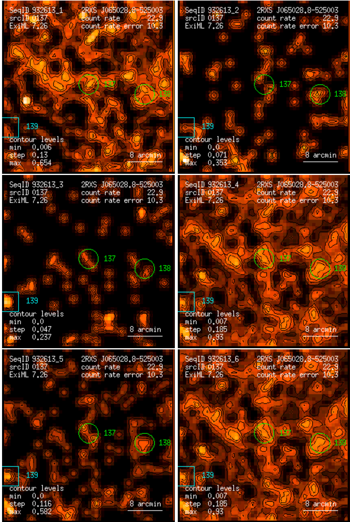
Figure 137: RASS 932613: detection 0137: band rate images, Gaussian filter: (1) PSPC channels 11 – 41, (2) 52 – 90, (3) 91 – 201, (4) 11 – 235, (5) 52 – 201, (6) 11 – 201. Broad band rates in counts/ks. Band rate contour levels in counts/ks/arcmin 2 .
