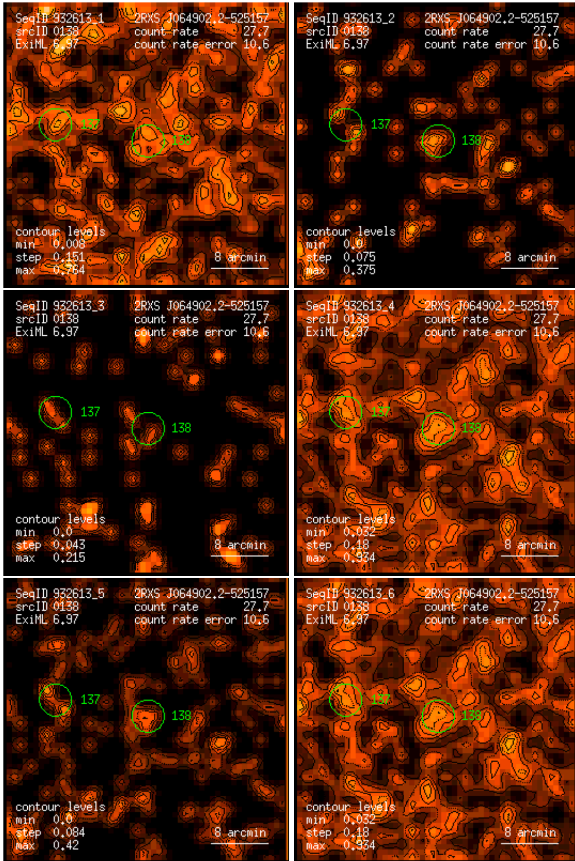
Figure 138: RASS 932613: detection 0138: band rate images, Gaussian filter: (1) PSPC channels 11 – 41, (2) 52 – 90, (3) 91 – 201, (4) 11 – 235, (5) 52 – 201, (6) 11 – 201. Broad band rates in counts/ks. Band rate contour levels in counts/ks/arcmin 2 .
