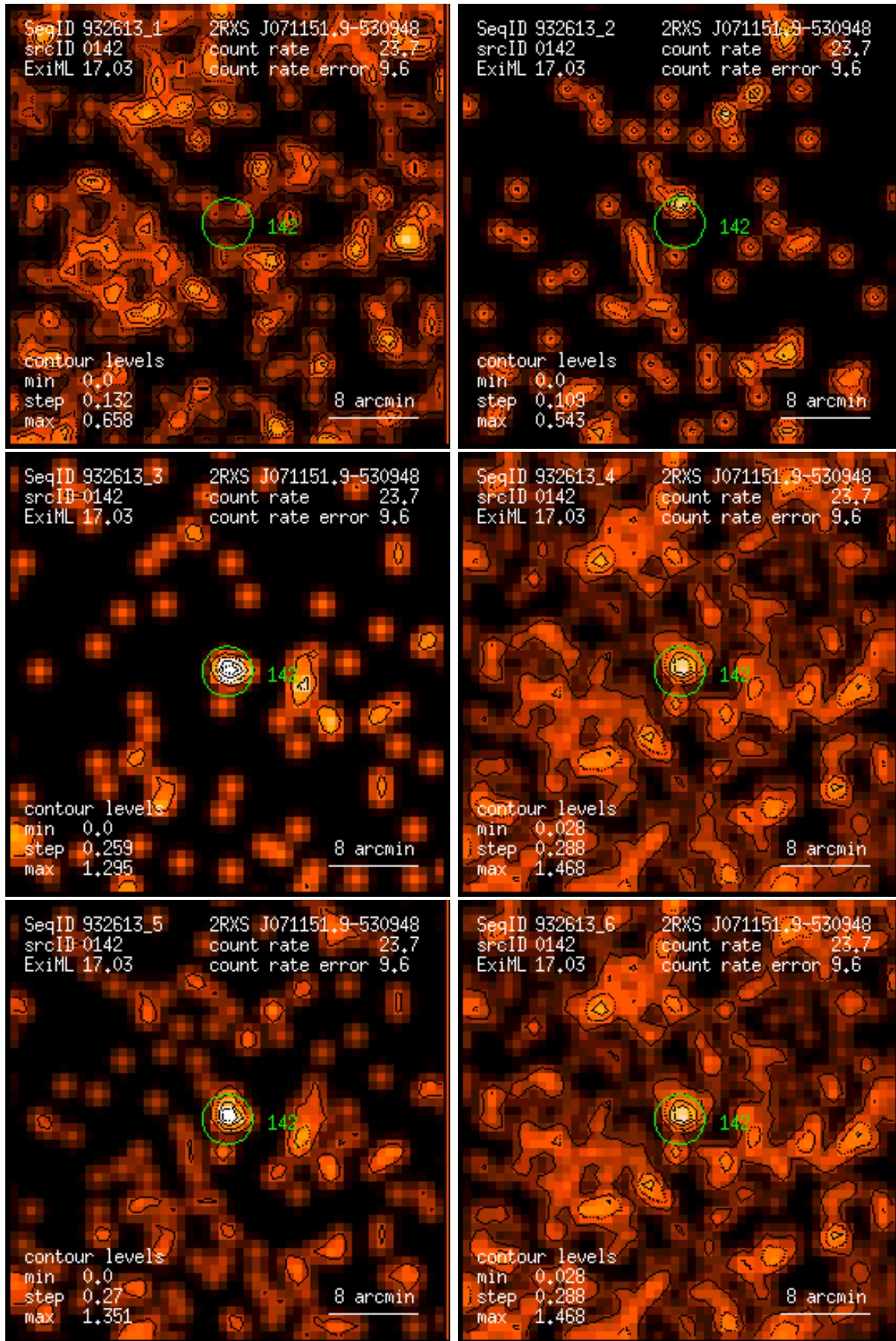
Figure 142: RASS 932613: detection 0142: band rate images, Gaussian filter: (1) PSPC channels 11 – 41, (2) 52 – 90, (3) 91 – 201, (4) 11 – 235, (5) 52 – 201, (6) 11 – 201. Broad band rates in counts/ks. Band rate contour levels in counts/ks/arcmin 2 .
