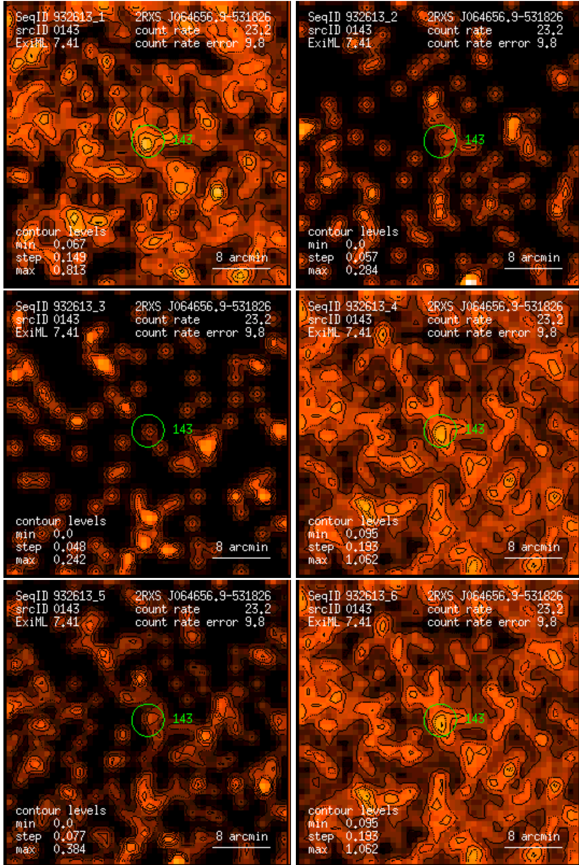
Figure 143: RASS 932613: detection 0143: band rate images, Gaussian filter: (1) PSPC channels 11 – 41, (2) 52 – 90, (3) 91 – 201, (4) 11 – 235, (5) 52 – 201, (6) 11 – 201. Broad band rates in counts/ks. Band rate contour levels in counts/ks/arcmin 2 .
