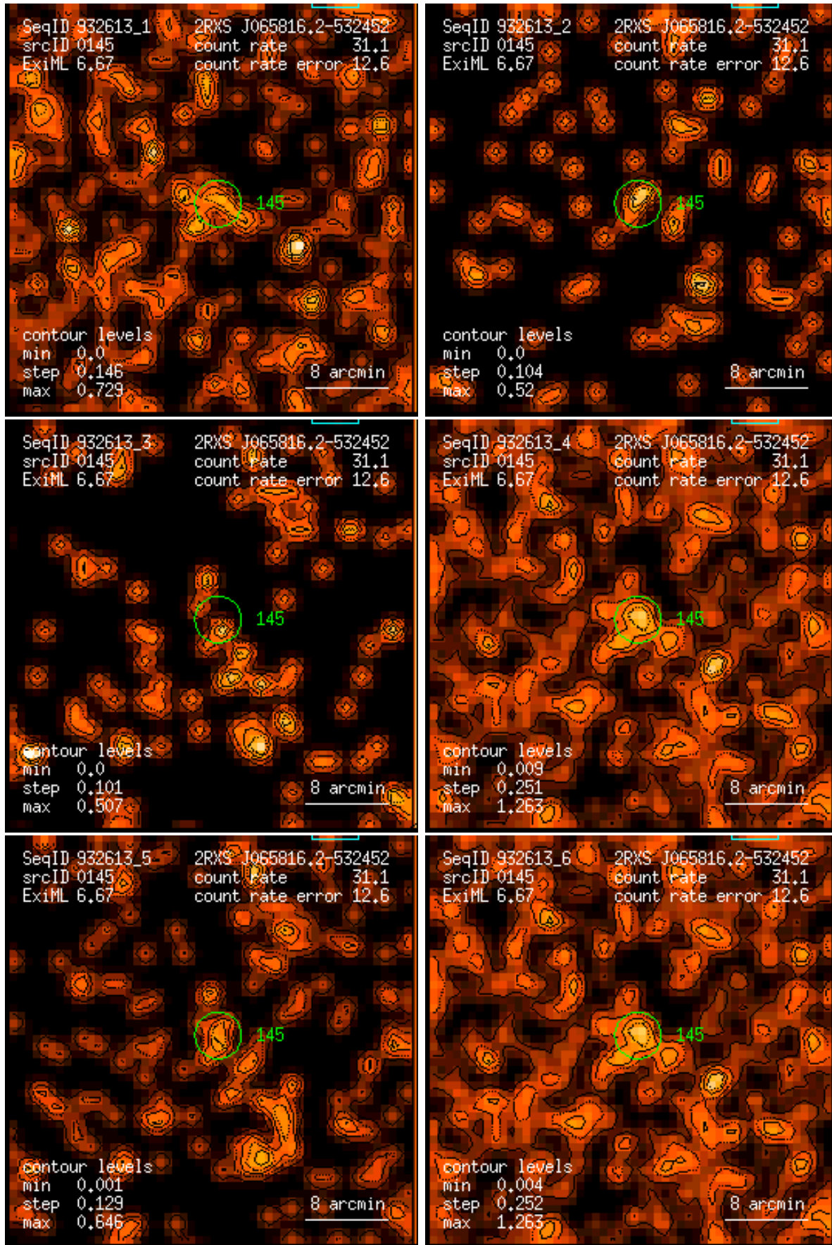
Figure 145: RASS 932613: detection 0145: band rate images, Gaussian filter: (1) PSPC channels 11 – 41, (2) 52 – 90, (3) 91 – 201, (4) 11 – 235, (5) 52 – 201, (6) 11 – 201. Broad band rates in counts/ks. Band rate contour levels in counts/ks/arcmin 2 .
