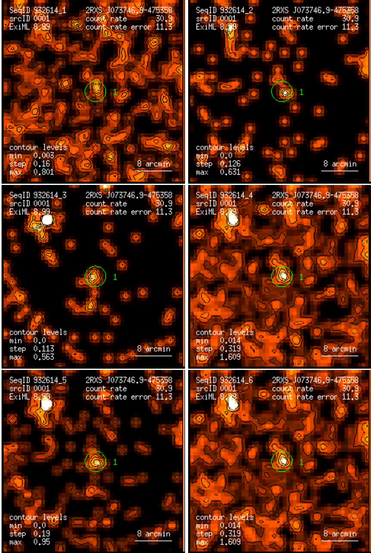
Figure 1: RASS 932614: detection 0001: band rate images, Gaussian filter: (1) PSPC channels 11 – 41, (2) 52 – 90, (3) 91 – 201, (4) 11 – 235, (5) 52 – 201, (6) 11 – 201. Broad band rates in counts/ks. Band rate contour levels in counts/ks/arcmin 2 .
