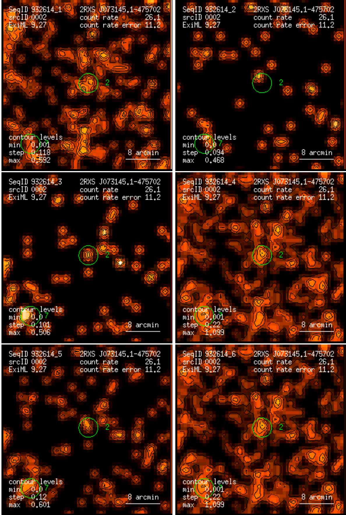
Figure 2: RASS 932614: detection 0002: band rate images, Gaussian filter: (1) PSPC channels 11 – 41, (2) 52 – 90, (3) 91 – 201, (4) 11 – 235, (5) 52 – 201, (6) 11 – 201. Broad band rates in counts/ks. Band rate contour levels in counts/ks/arcmin 2 .
