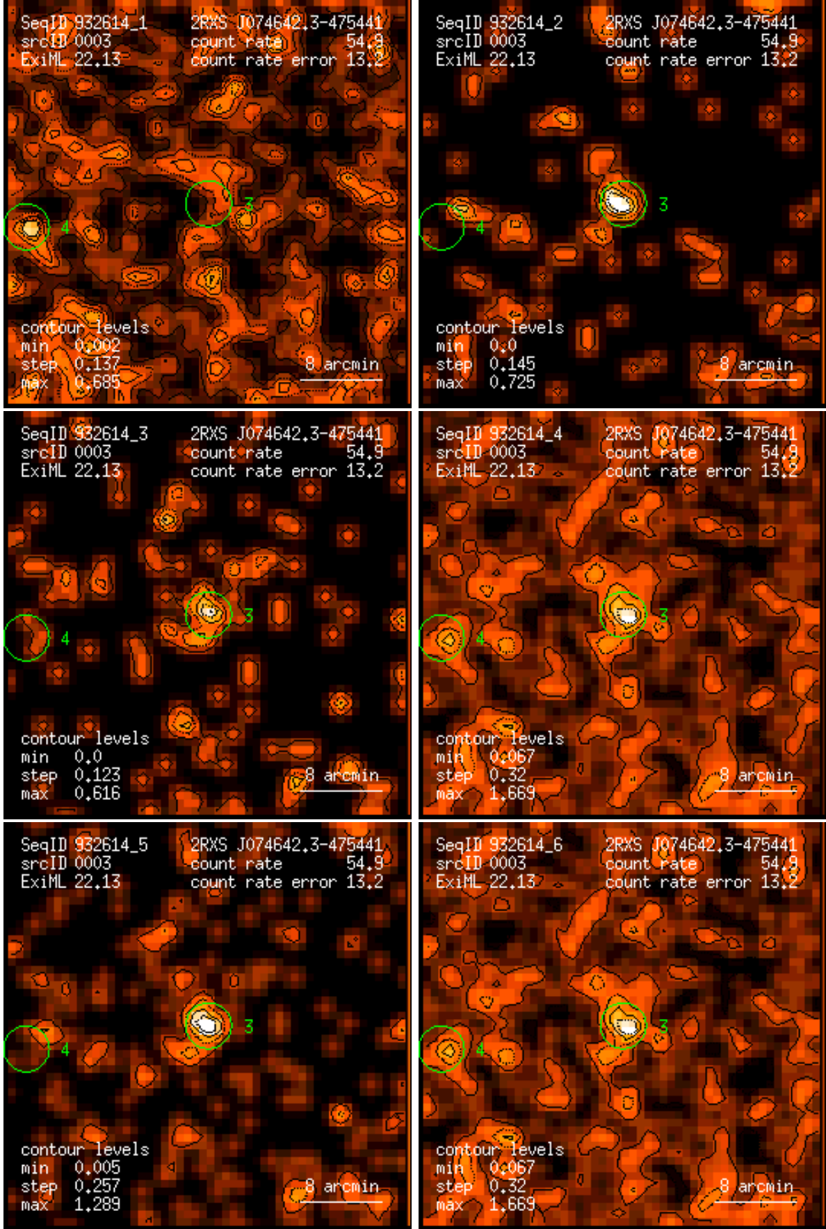
Figure 3: RASS 932614: detection 0003: band rate images, Gaussian filter: (1) PSPC channels 11 – 41, (2) 52 – 90, (3) 91 – 201, (4) 11 – 235, (5) 52 – 201, (6) 11 – 201. Broad band rates in counts/ks. Band rate contour levels in counts/ks/arcmin 2 .
