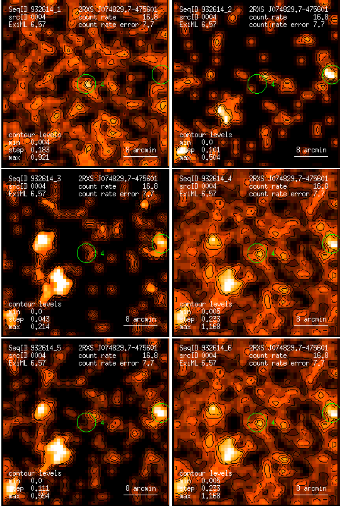
Figure 4: RASS 932614: detection 0004: band rate images, Gaussian filter: (1) PSPC channels 11 – 41, (2) 52 – 90, (3) 91 – 201, (4) 11 – 235, (5) 52 – 201, (6) 11 – 201. Broad band rates in counts/ks. Band rate contour levels in counts/ks/arcmin 2 .
