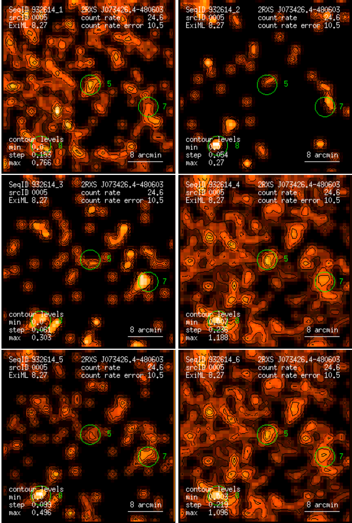
Figure 5: RASS 932614: detection 0005: band rate images, Gaussian filter: (1) PSPC channels 11 – 41, (2) 52 – 90, (3) 91 – 201, (4) 11 – 235, (5) 52 – 201, (6) 11 – 201. Broad band rates in counts/ks. Band rate contour levels in counts/ks/arcmin 2 .
