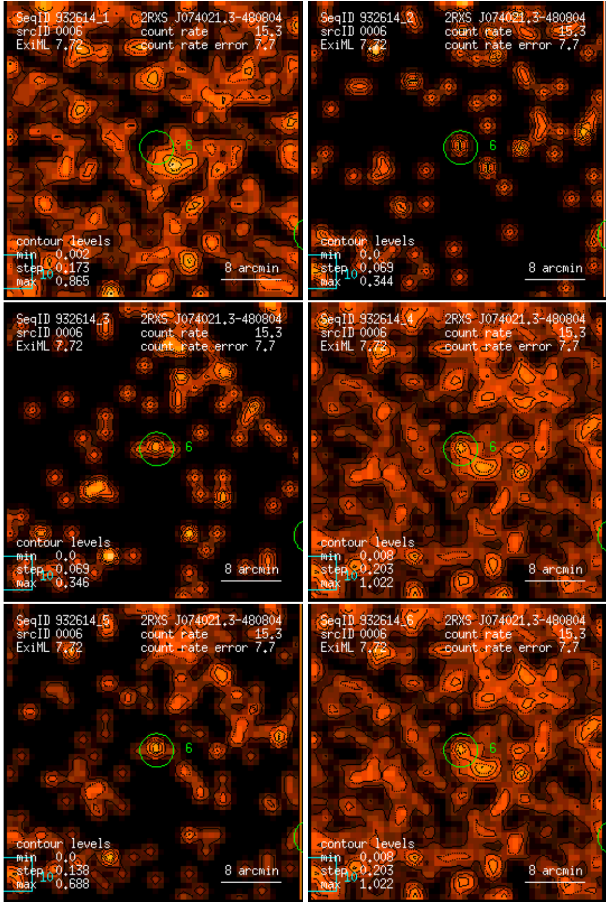
Figure 6: RASS 932614: detection 0006: band rate images, Gaussian filter: (1) PSPC channels 11 – 41, (2) 52 – 90, (3) 91 – 201, (4) 11 – 235, (5) 52 – 201, (6) 11 – 201. Broad band rates in counts/ks. Band rate contour levels in counts/ks/arcmin 2 .
