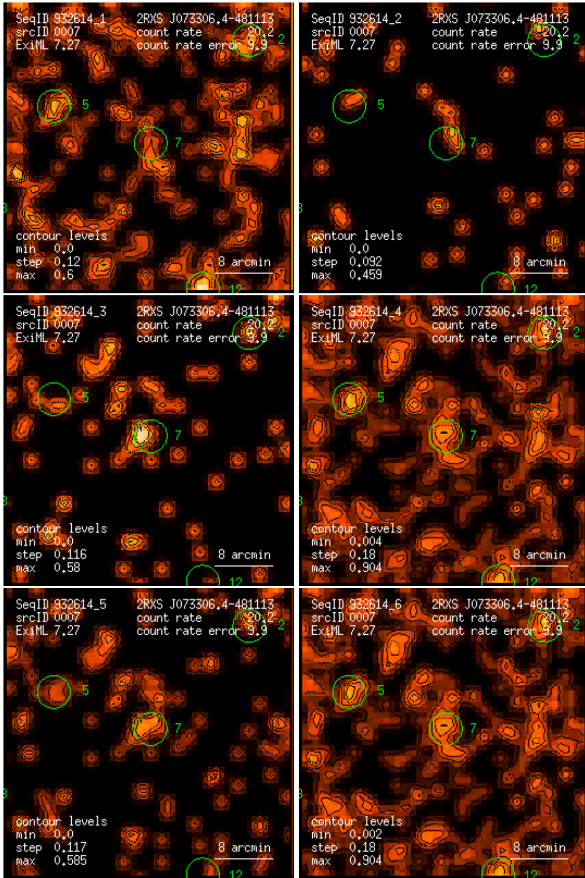
Figure 7: RASS 932614: detection 0007: band rate images, Gaussian filter: (1) PSPC channels 11 – 41, (2) 52 – 90, (3) 91 – 201, (4) 11 – 235, (5) 52 – 201, (6) 11 – 201. Broad band rates in counts/ks. Band rate contour levels in counts/ks/arcmin 2 .
