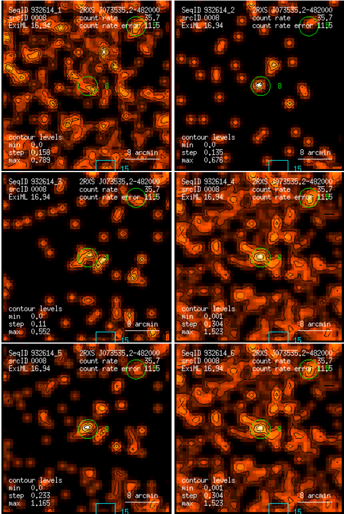
Figure 8: RASS 932614: detection 0008: band rate images, Gaussian filter: (1) PSPC channels 11 – 41, (2) 52 – 90, (3) 91 – 201, (4) 11 – 235, (5) 52 – 201, (6) 11 – 201. Broad band rates in counts/ks. Band rate contour levels in counts/ks/arcmin 2 .
