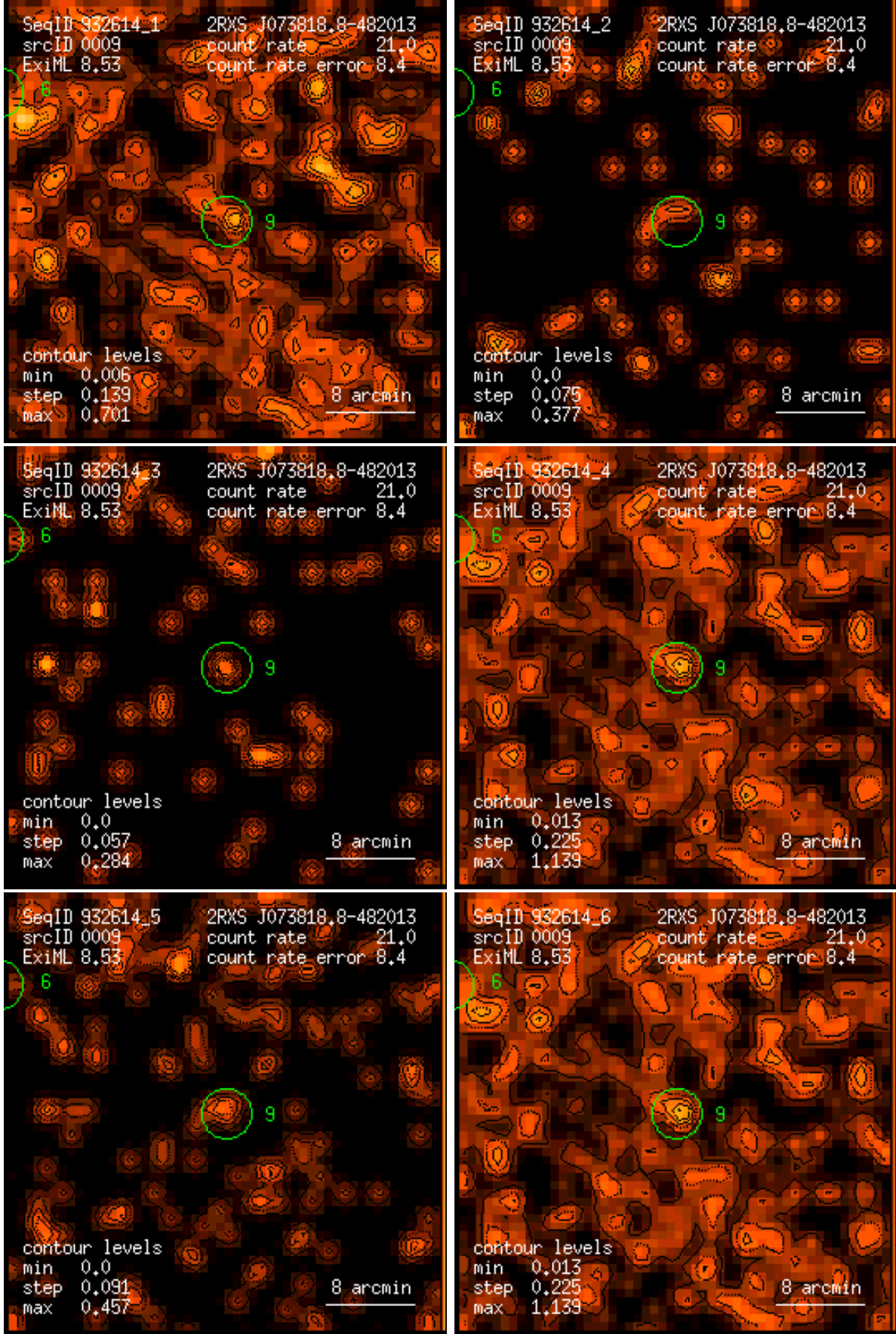
Figure 9: RASS 932614: detection 0009: band rate images, Gaussian filter: (1) PSPC channels 11 – 41, (2) 52 – 90, (3) 91 – 201, (4) 11 – 235, (5) 52 – 201, (6) 11 – 201. Broad band rates in counts/ks. Band rate contour levels in counts/ks/arcmin 2 .
