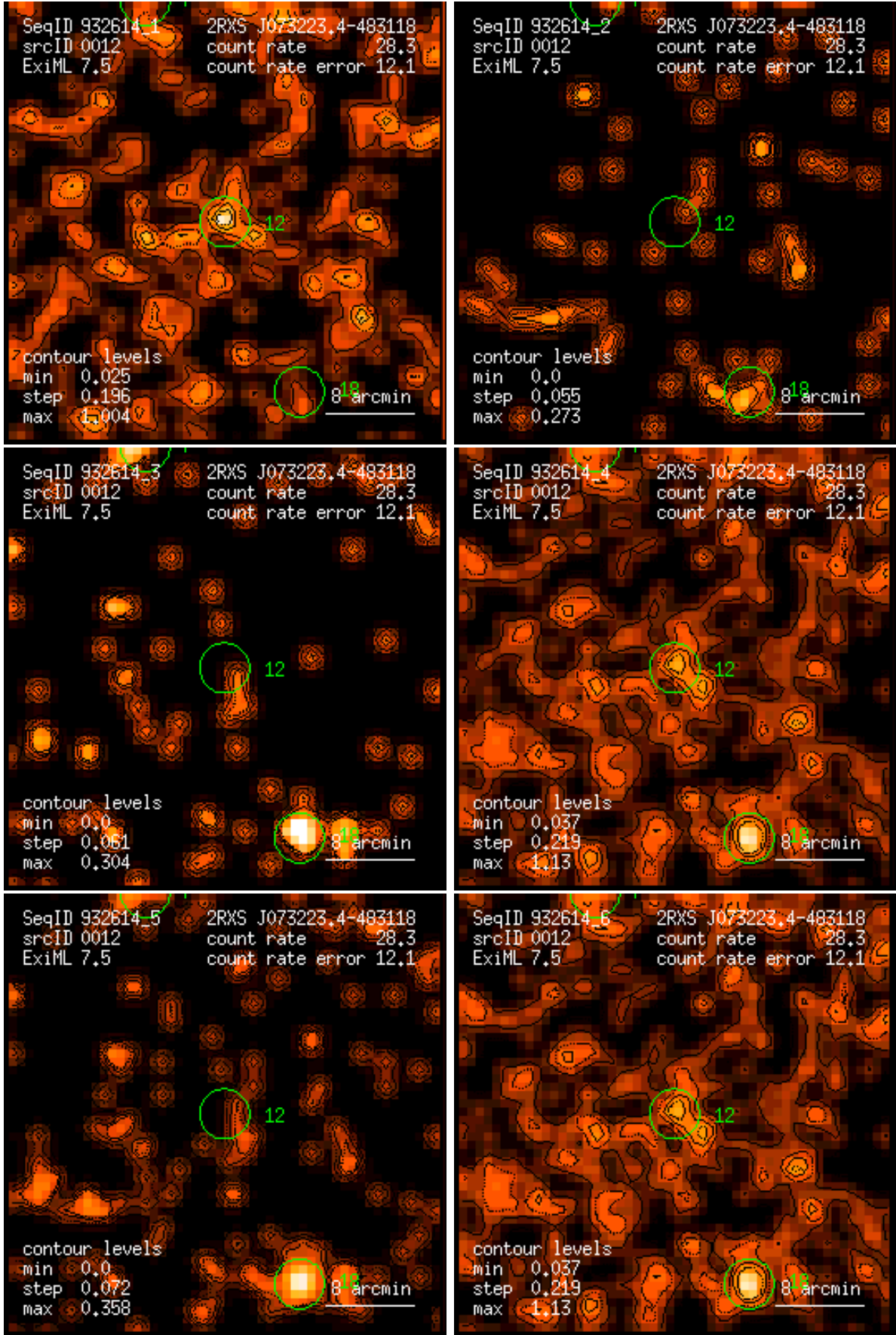
Figure 12: RASS 932614: detection 0012: band rate images, Gaussian filter: (1) PSPC channels 11 – 41, (2) 52 – 90, (3) 91 – 201, (4) 11 – 235, (5) 52 – 201, (6) 11 – 201. Broad band rates in counts/ks. Band rate contour levels in counts/ks/arcmin 2 .
