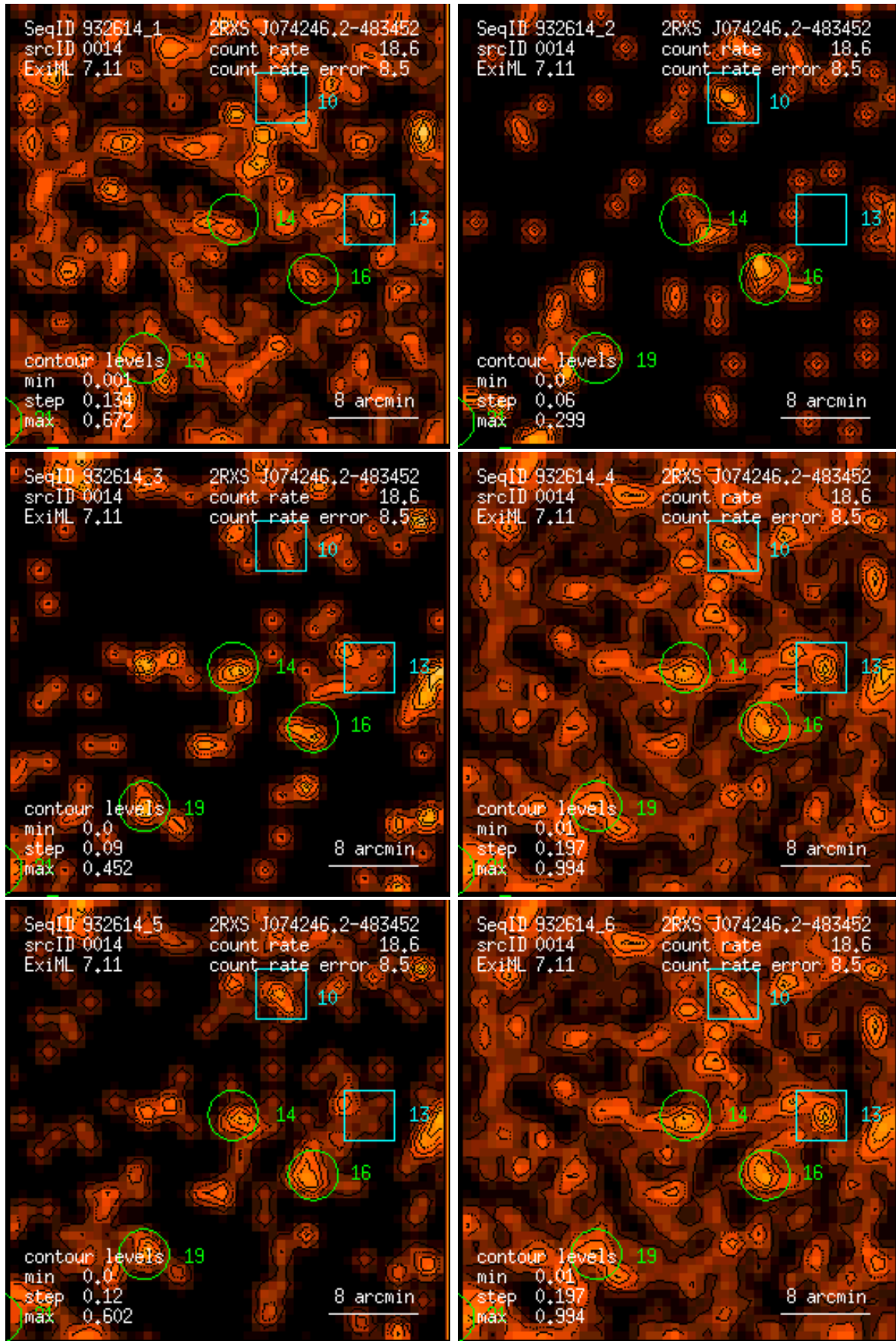
Figure 14: RASS 932614: detection 0014: band rate images, Gaussian filter: (1) PSPC channels 11 – 41, (2) 52 – 90, (3) 91 – 201, (4) 11 – 235, (5) 52 – 201, (6) 11 – 201. Broad band rates in counts/ks. Band rate contour levels in counts/ks/arcmin 2 .
