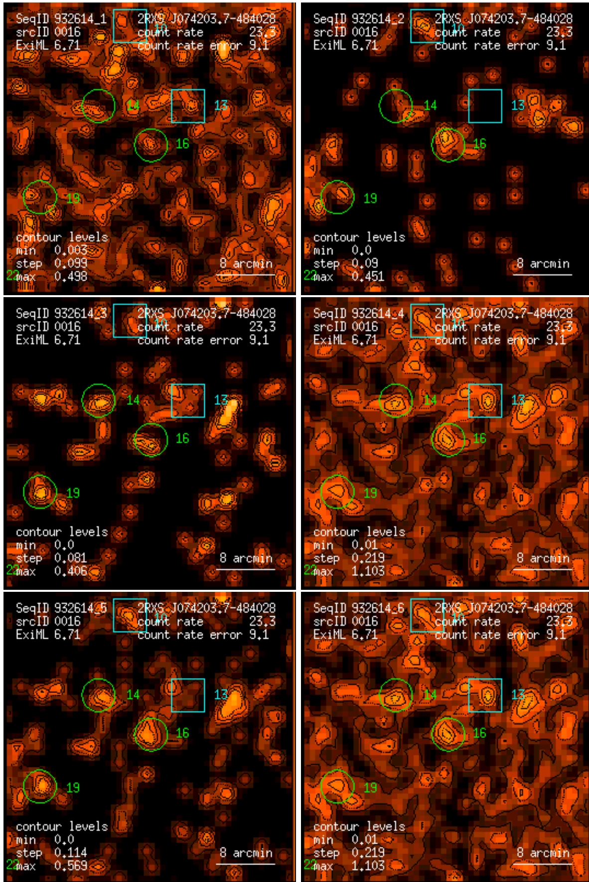
Figure 16: RASS 932614: detection 0016: band rate images, Gaussian filter: (1) PSPC channels 11 – 41, (2) 52 – 90, (3) 91 – 201, (4) 11 – 235, (5) 52 – 201, (6) 11 – 201. Broad band rates in counts/ks. Band rate contour levels in counts/ks/arcmin 2 .
