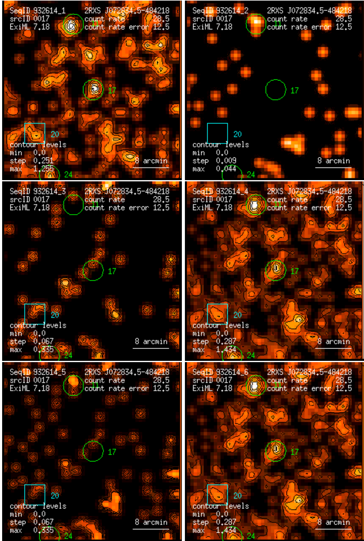
Figure 17: RASS 932614: detection 0017: band rate images, Gaussian filter: (1) PSPC channels 11 – 41, (2) 52 – 90, (3) 91 – 201, (4) 11 – 235, (5) 52 – 201, (6) 11 – 201. Broad band rates in counts/ks. Band rate contour levels in counts/ks/arcmin 2 .
