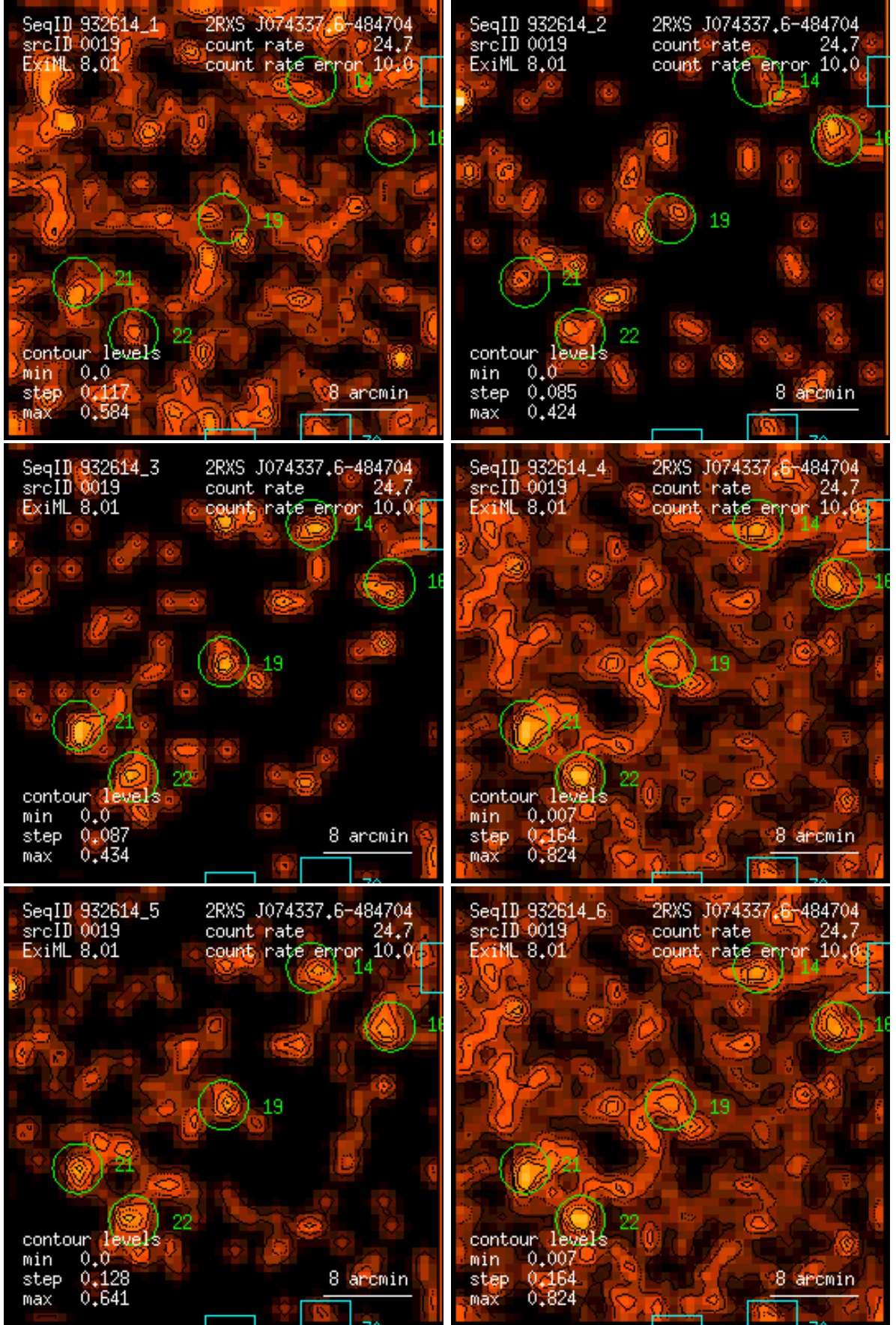
Figure 19: RASS 932614: detection 0019: band rate images, Gaussian filter: (1) PSPC channels 11 – 41, (2) 52 – 90, (3) 91 – 201, (4) 11 – 235, (5) 52 – 201, (6) 11 – 201. Broad band rates in counts/ks. Band rate contour levels in counts/ks/arcmin 2 .
