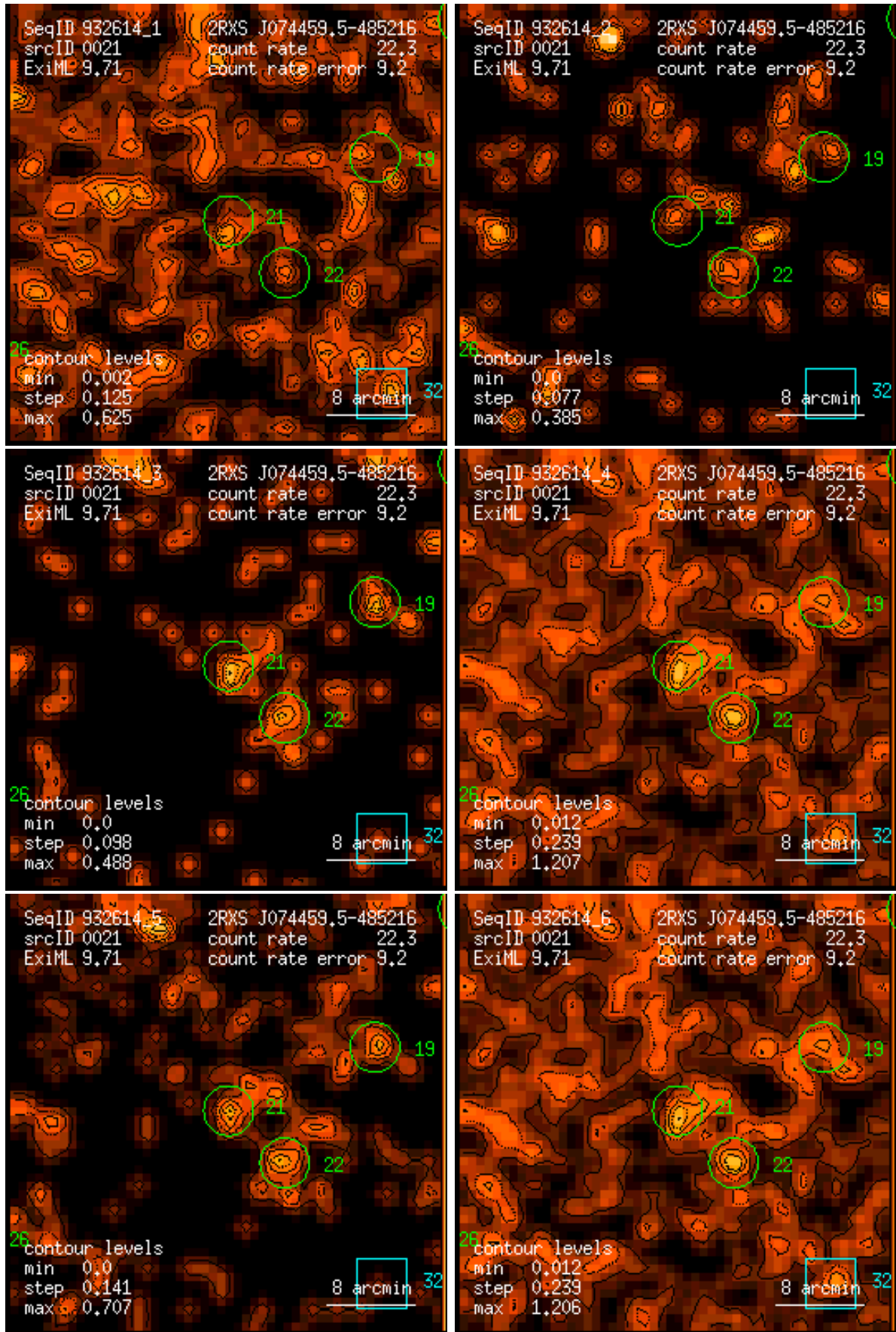
Figure 21: RASS 932614: detection 0021: band rate images, Gaussian filter: (1) PSPC channels 11 – 41, (2) 52 – 90, (3) 91 – 201, (4) 11 – 235, (5) 52 – 201, (6) 11 – 201. Broad band rates in counts/ks. Band rate contour levels in counts/ks/arcmin 2 .
