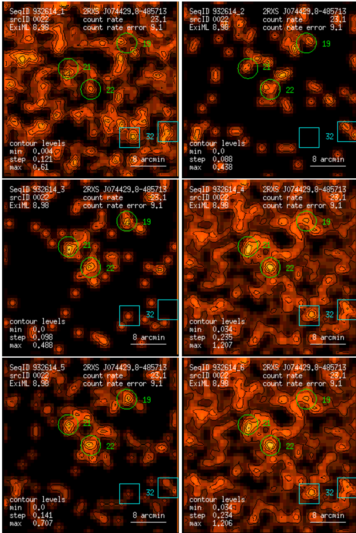
Figure 22: RASS 932614: detection 0022: band rate images, Gaussian filter: (1) PSPC channels 11 – 41, (2) 52 – 90, (3) 91 – 201, (4) 11 – 235, (5) 52 – 201, (6) 11 – 201. Broad band rates in counts/ks. Band rate contour levels in counts/ks/arcmin 2 .
