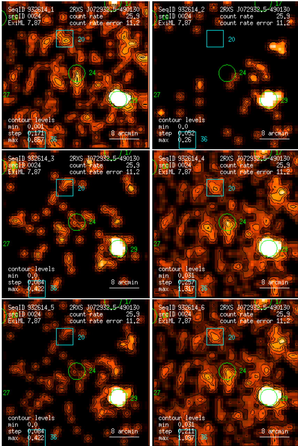
Figure 24: RASS 932614: detection 0024: band rate images, Gaussian filter: (1) PSPC channels 11 – 41, (2) 52 – 90, (3) 91 – 201, (4) 11 – 235, (5) 52 – 201, (6) 11 – 201. Broad band rates in counts/ks. Band rate contour levels in counts/ks/arcmin 2 .
