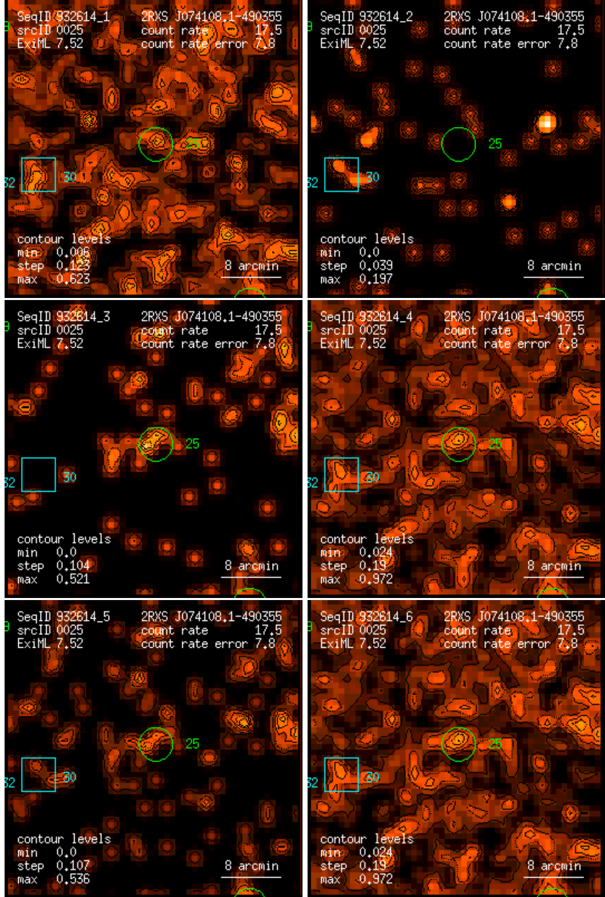
Figure 25: RASS 932614: detection 0025: band rate images, Gaussian filter: (1) PSPC channels 11 – 41, (2) 52 – 90, (3) 91 – 201, (4) 11 – 235, (5) 52 – 201, (6) 11 – 201. Broad band rates in counts/ks. Band rate contour levels in counts/ks/arcmin 2 .
