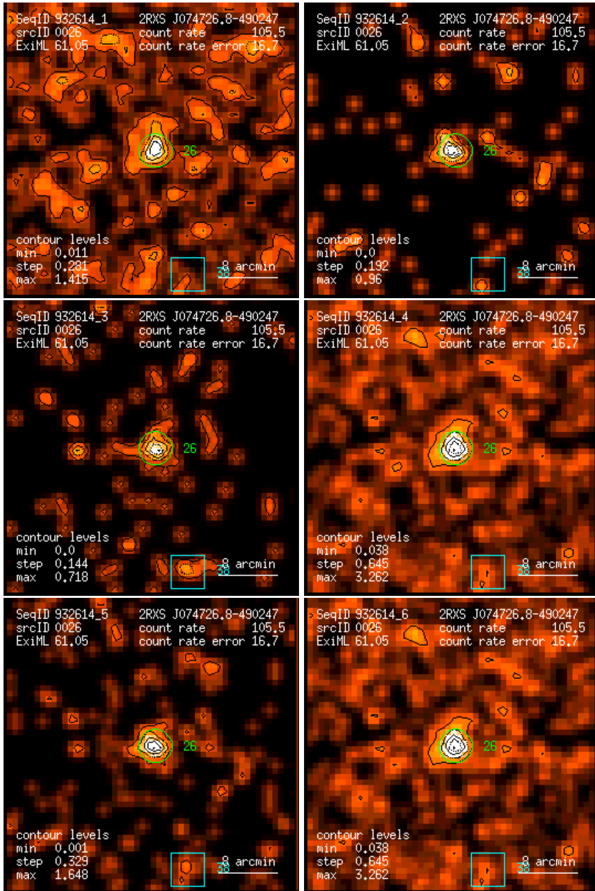
Figure 26: RASS 932614: detection 0026: band rate images, Gaussian filter: (1) PSPC channels 11 – 41, (2) 52 – 90, (3) 91 – 201, (4) 11 – 235, (5) 52 – 201, (6) 11 – 201. Broad band rates in counts/ks. Band rate contour levels in counts/ks/arcmin 2 .
