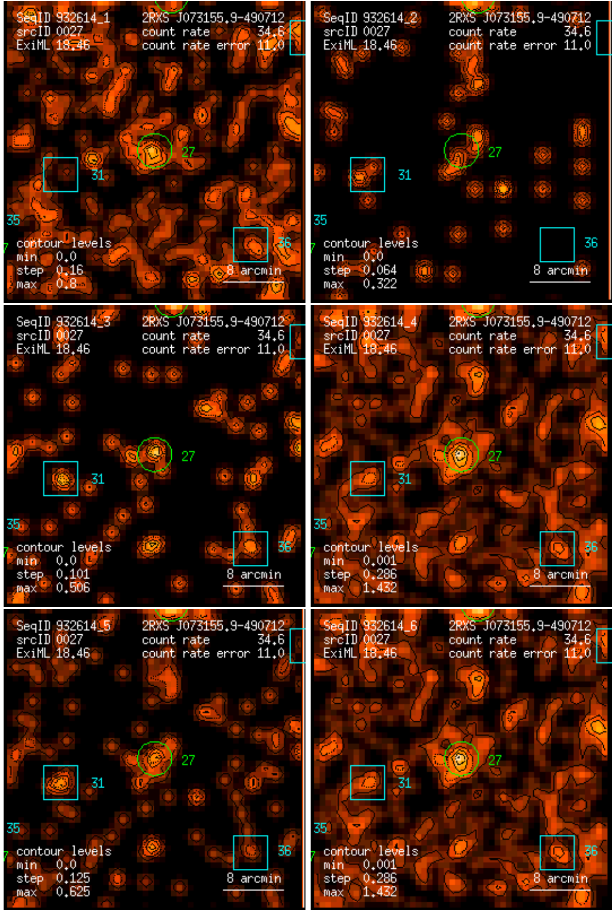
Figure 27: RASS 932614: detection 0027: band rate images, Gaussian filter: (1) PSPC channels 11 – 41, (2) 52 – 90, (3) 91 – 201, (4) 11 – 235, (5) 52 – 201, (6) 11 – 201. Broad band rates in counts/ks. Band rate contour levels in counts/ks/arcmin 2 .
