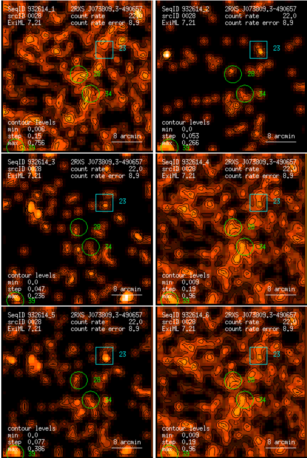
Figure 28: RASS 932614: detection 0028: band rate images, Gaussian filter: (1) PSPC channels 11 – 41, (2) 52 – 90, (3) 91 – 201, (4) 11 – 235, (5) 52 – 201, (6) 11 – 201. Broad band rates in counts/ks. Band rate contour levels in counts/ks/arcmin 2 .
