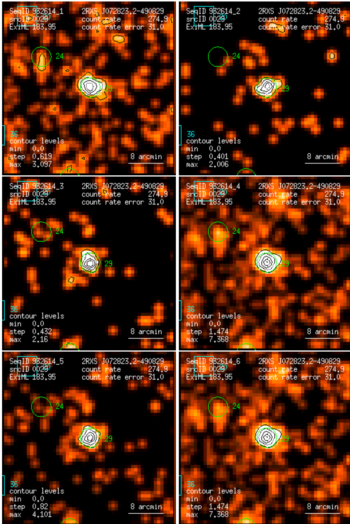
Figure 29: RASS 932614: detection 0029: band rate images, Gaussian filter: (1) PSPC channels 11 – 41, (2) 52 – 90, (3) 91 – 201, (4) 11 – 235, (5) 52 – 201, (6) 11 – 201. Broad band rates in counts/ks. Band rate contour levels in counts/ks/arcmin 2 .
