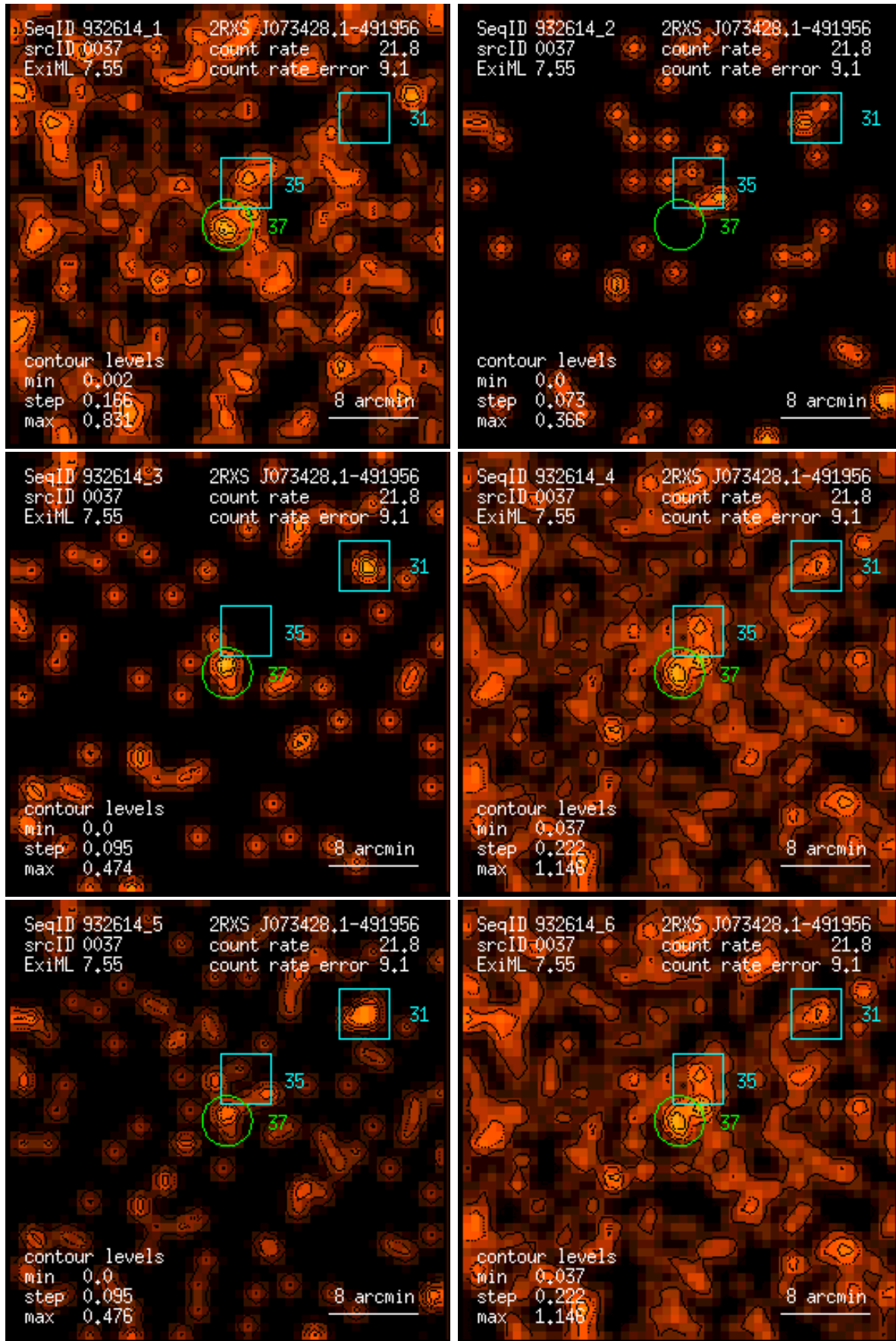
Figure 37: RASS 932614: detection 0037: band rate images, Gaussian filter: (1) PSPC channels 11 – 41, (2) 52 – 90, (3) 91 – 201, (4) 11 – 235, (5) 52 – 201, (6) 11 – 201. Broad band rates in counts/ks. Band rate contour levels in counts/ks/arcmin 2 .
