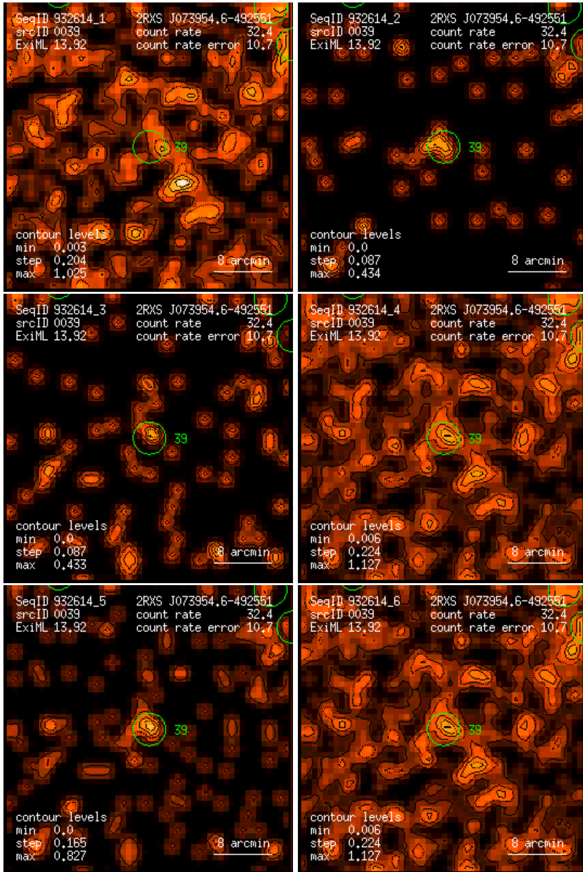
Figure 39: RASS 932614: detection 0039: band rate images, Gaussian filter: (1) PSPC channels 11 – 41, (2) 52 – 90, (3) 91 – 201, (4) 11 – 235, (5) 52 – 201, (6) 11 – 201. Broad band rates in counts/ks. Band rate contour levels in counts/ks/arcmin 2 .
