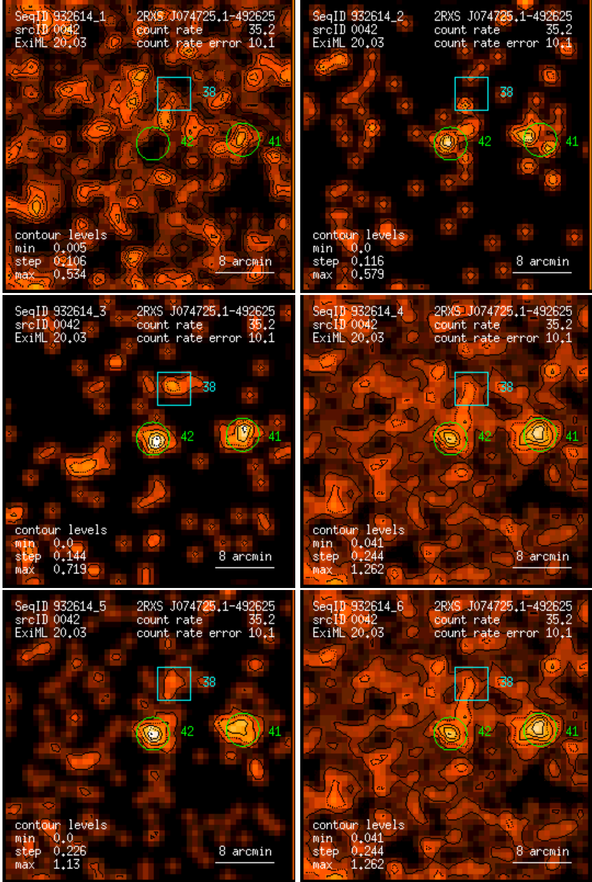
Figure 42: RASS 932614: detection 0042: band rate images, Gaussian filter: (1) PSPC channels 11 – 41, (2) 52 – 90, (3) 91 – 201, (4) 11 – 235, (5) 52 – 201, (6) 11 – 201. Broad band rates in counts/ks. Band rate contour levels in counts/ks/arcmin 2 .
