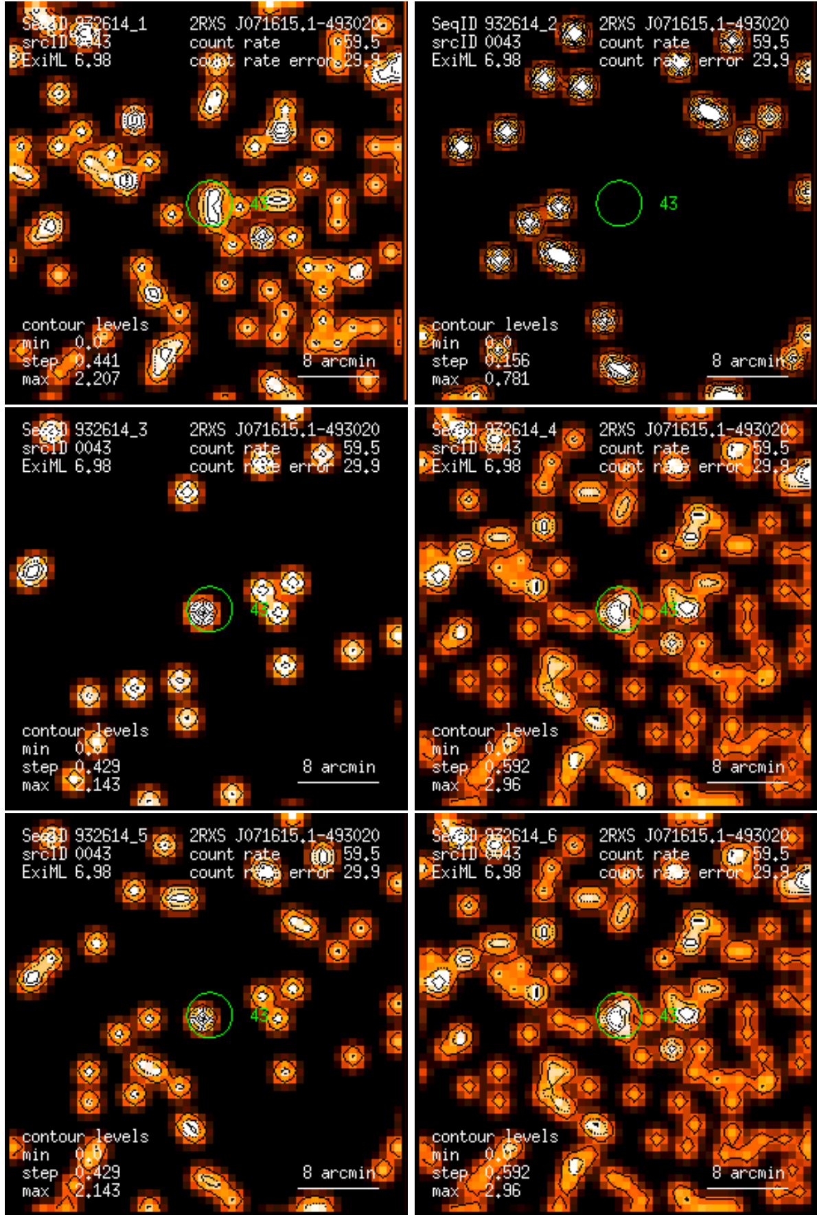
Figure 43: RASS 932614: detection 0043: band rate images, Gaussian filter: (1) PSPC channels 11 – 41, (2) 52 – 90, (3) 91 – 201, (4) 11 – 235, (5) 52 – 201, (6) 11 – 201. Broad band rates in counts/ks. Band rate contour levels in counts/ks/arcmin 2 .
