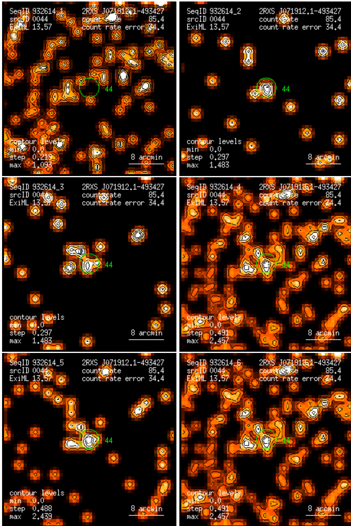
Figure 44: RASS 932614: detection 0044: band rate images, Gaussian filter: (1) PSPC channels 11 – 41, (2) 52 – 90, (3) 91 – 201, (4) 11 – 235, (5) 52 – 201, (6) 11 – 201. Broad band rates in counts/ks. Band rate contour levels in counts/ks/arcmin 2 .
