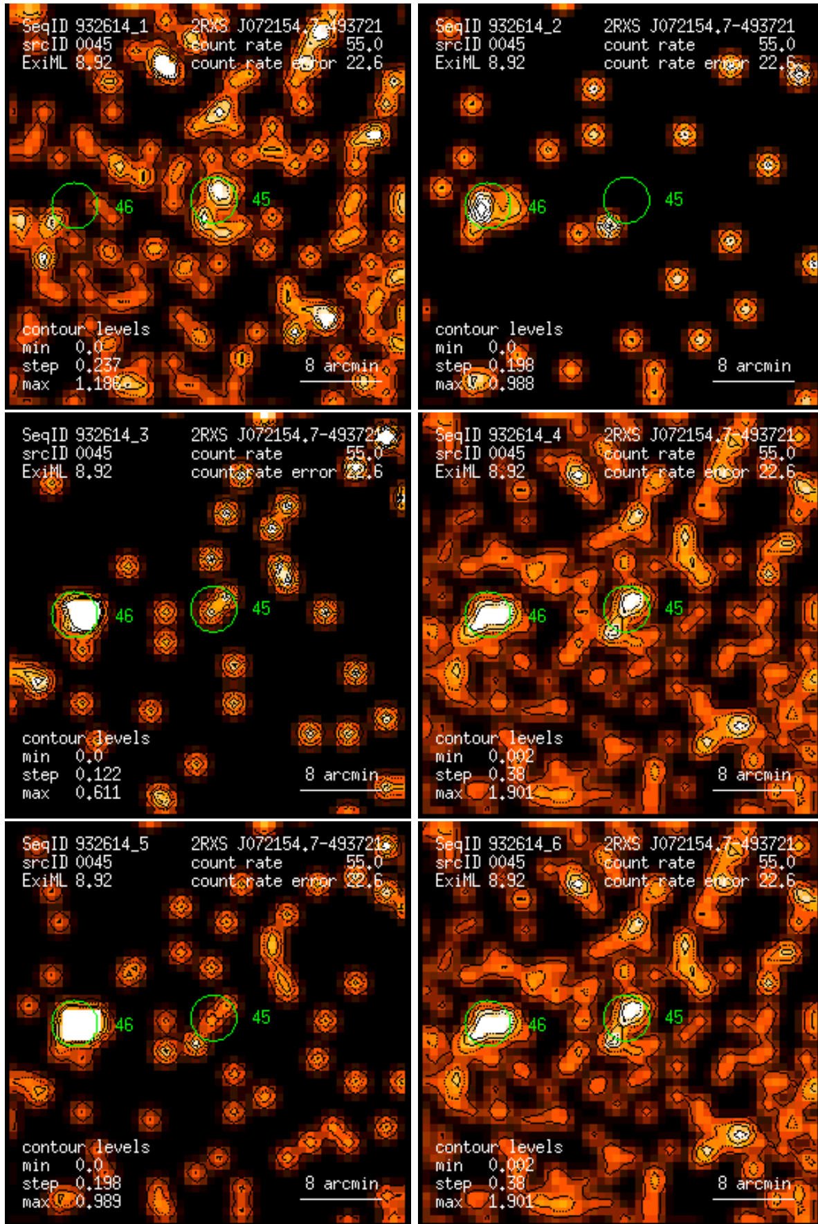
Figure 45: RASS 932614: detection 0045: band rate images, Gaussian filter: (1) PSPC channels 11 – 41, (2) 52 – 90, (3) 91 – 201, (4) 11 – 235, (5) 52 – 201, (6) 11 – 201. Broad band rates in counts/ks. Band rate contour levels in counts/ks/arcmin 2 .
