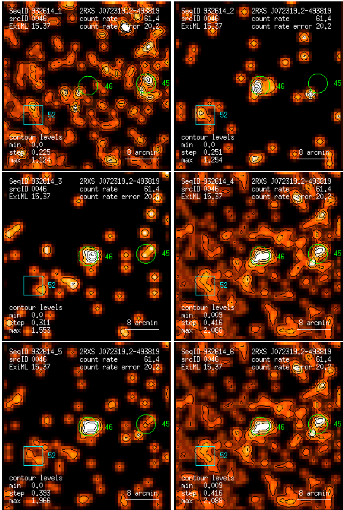
Figure 46: RASS 932614: detection 0046: band rate images, Gaussian filter: (1) PSPC channels 11 – 41, (2) 52 – 90, (3) 91 – 201, (4) 11 – 235, (5) 52 – 201, (6) 11 – 201. Broad band rates in counts/ks. Band rate contour levels in counts/ks/arcmin 2 .
