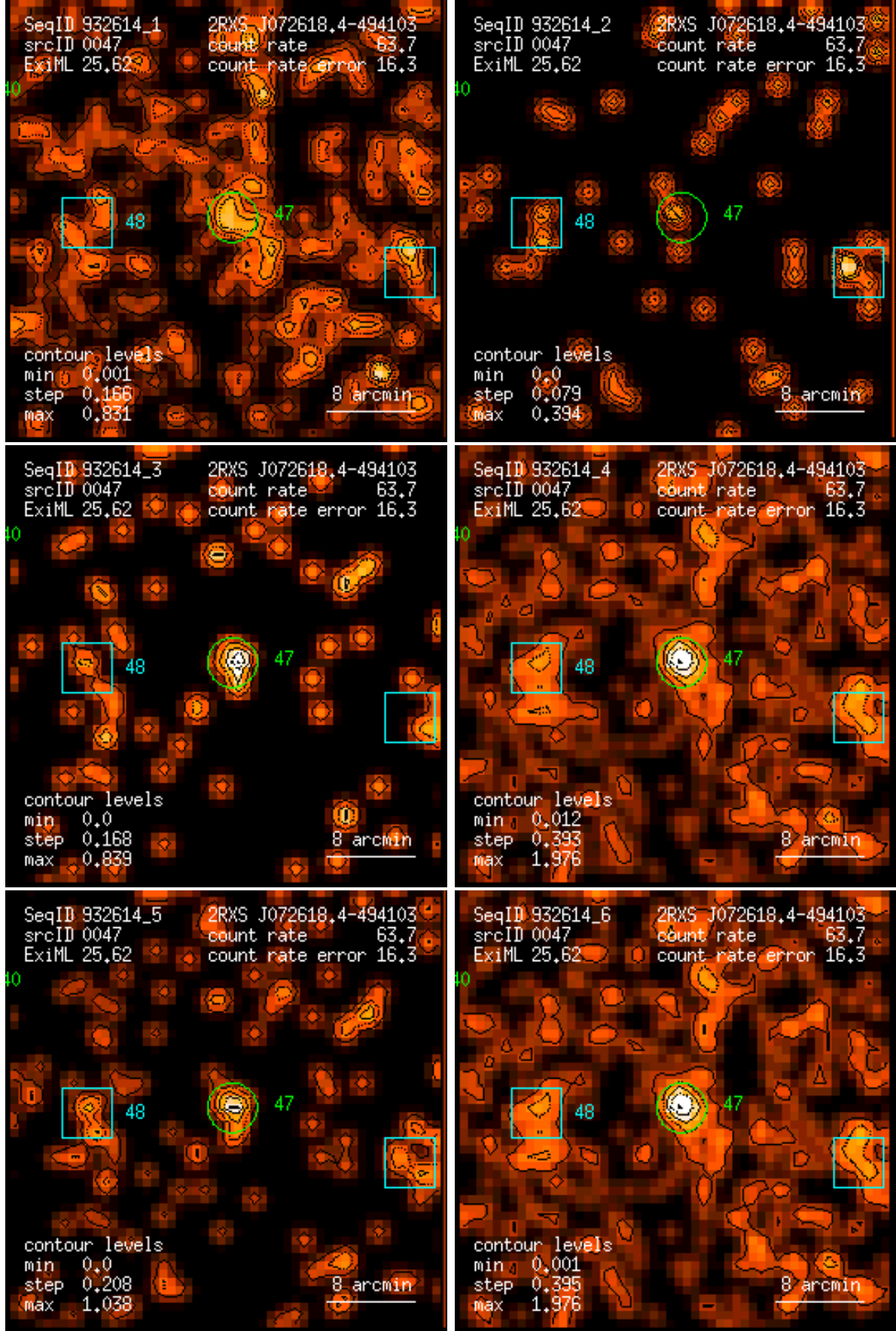
Figure 47: RASS 932614: detection 0047: band rate images, Gaussian filter: (1) PSPC channels 11 – 41, (2) 52 – 90, (3) 91 – 201, (4) 11 – 235, (5) 52 – 201, (6) 11 – 201. Broad band rates in counts/ks. Band rate contour levels in counts/ks/arcmin 2 .
