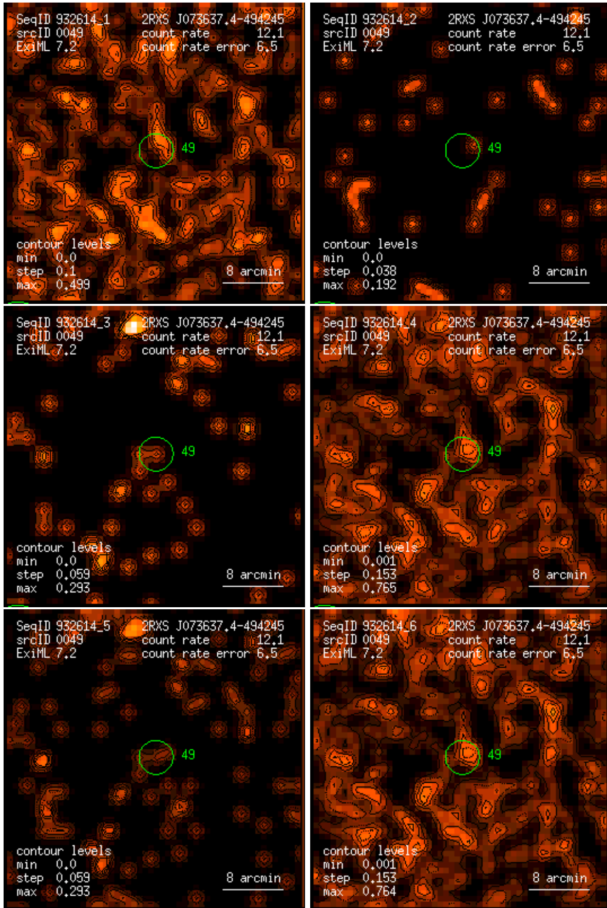
Figure 49: RASS 932614: detection 0049: band rate images, Gaussian filter: (1) PSPP channels 11 – 41, (2) 52 – 90, (3) 91 – 201, (4) 11 – 235, (5) 52 – 201, (6) 11 – 201. Broad band rates in counts/ks. Band rate contour levels in counts/ks/arcmin 2 .
