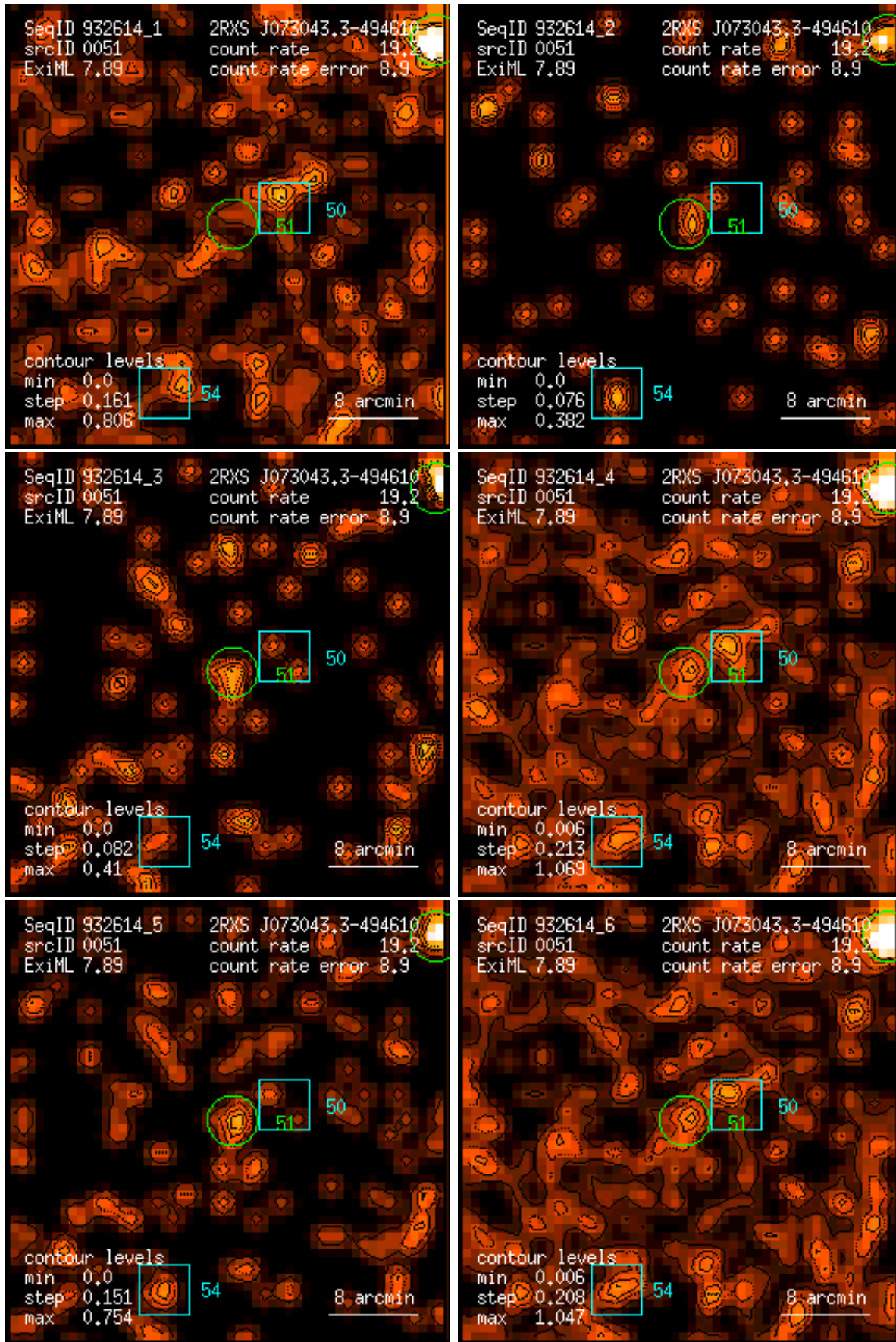
Figure 51: RASS 932614: detection 0051: band rate images, Gaussian filter: (1) PSPC channels 11 – 41, (2) 52 – 90, (3) 91 – 201, (4) 11 – 235, (5) 52 – 201, (6) 11 – 201. Broad band rates in counts/ks. Band rate contour levels in counts/ks/arcmin 2 .
