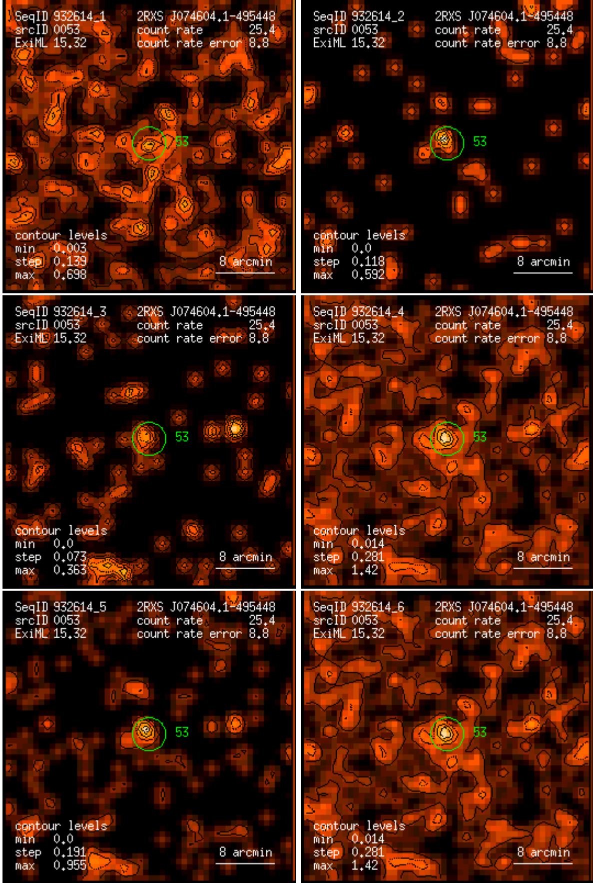
Figure 53: RASS 932614: detection 0053: band rate images, Gaussian filter: (1) PSPC channels 11 – 41, (2) 52 – 90, (3) 91 – 201, (4) 11 – 235, (5) 52 – 201, (6) 11 – 201. Broad band rates in counts/ks. Band rate contour levels in counts/ks/arcmin 2 .
