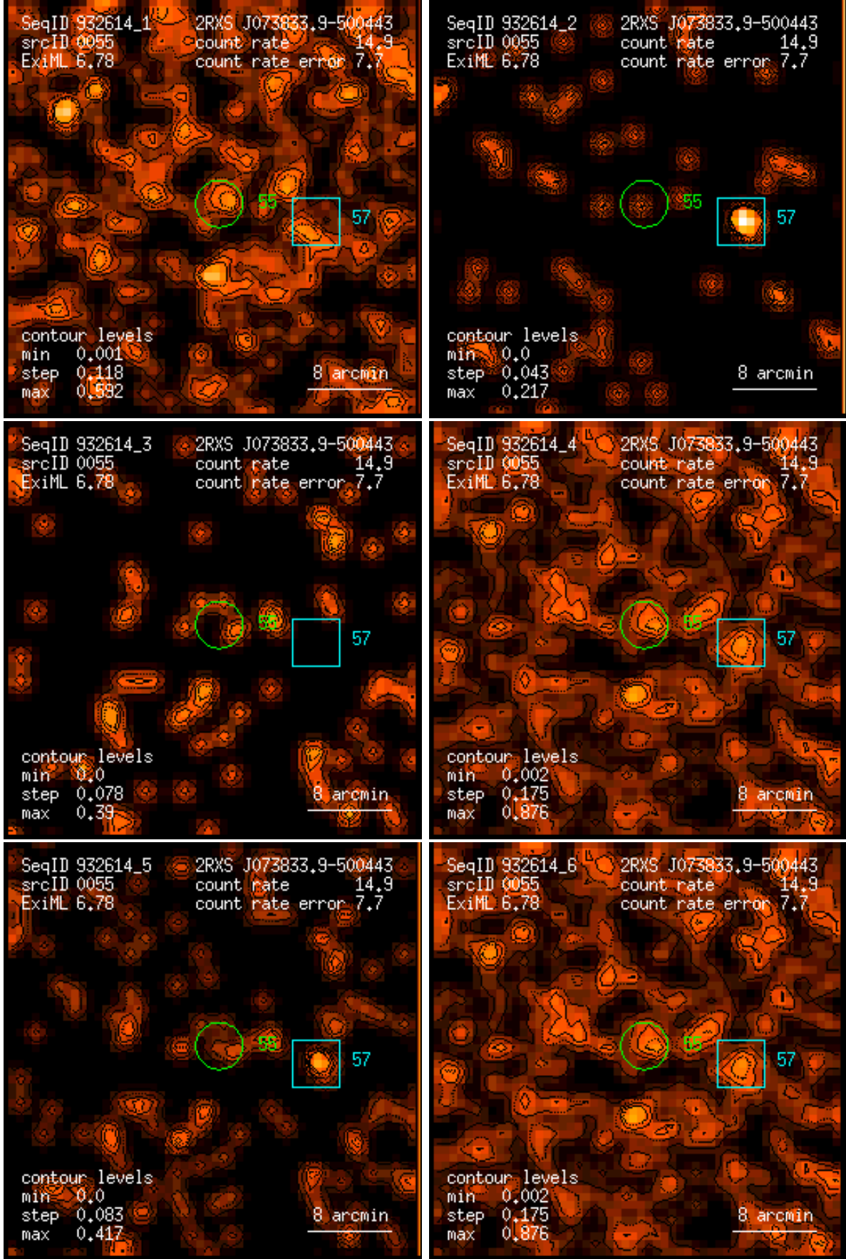
Figure 55: RASS 932614: detection 0055: band rate images, Gaussian filter: (1) PSPC channels 11 – 41, (2) 52 – 90, (3) 91 – 201, (4) 11 – 235, (5) 52 – 201, (6) 11 – 201. Broad band rates in counts/ks. Band rate contour levels in counts/ks/arcmin 2 .
