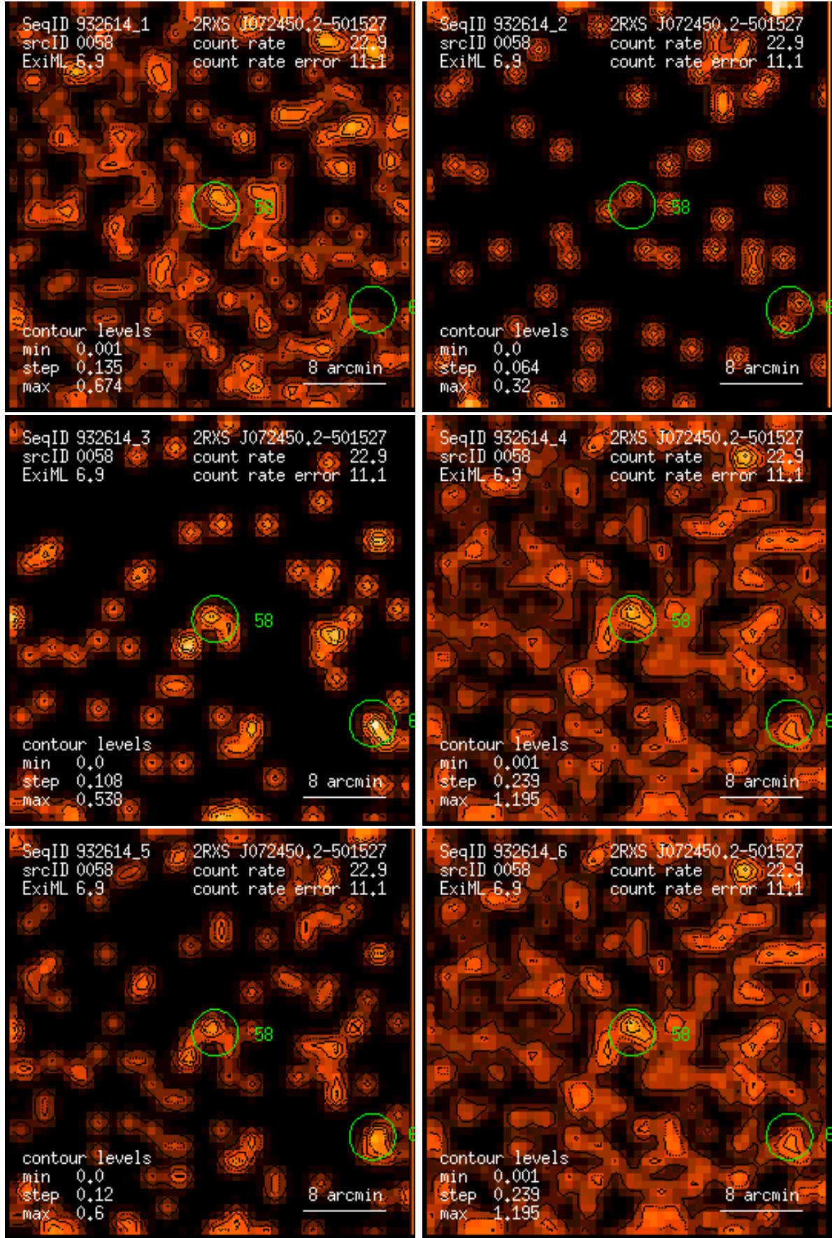
Figure 58: RASS 932614: detection 0058: band rate images, Gaussian filter: (1) PSPC channels 11 – 41, (2) 52 – 90, (3) 91 – 201, (4) 11 – 235, (5) 52 – 201, (6) 11 – 201. Broad band rates in counts/ks. Band rate contour levels in counts/ks/arcmin 2 .
